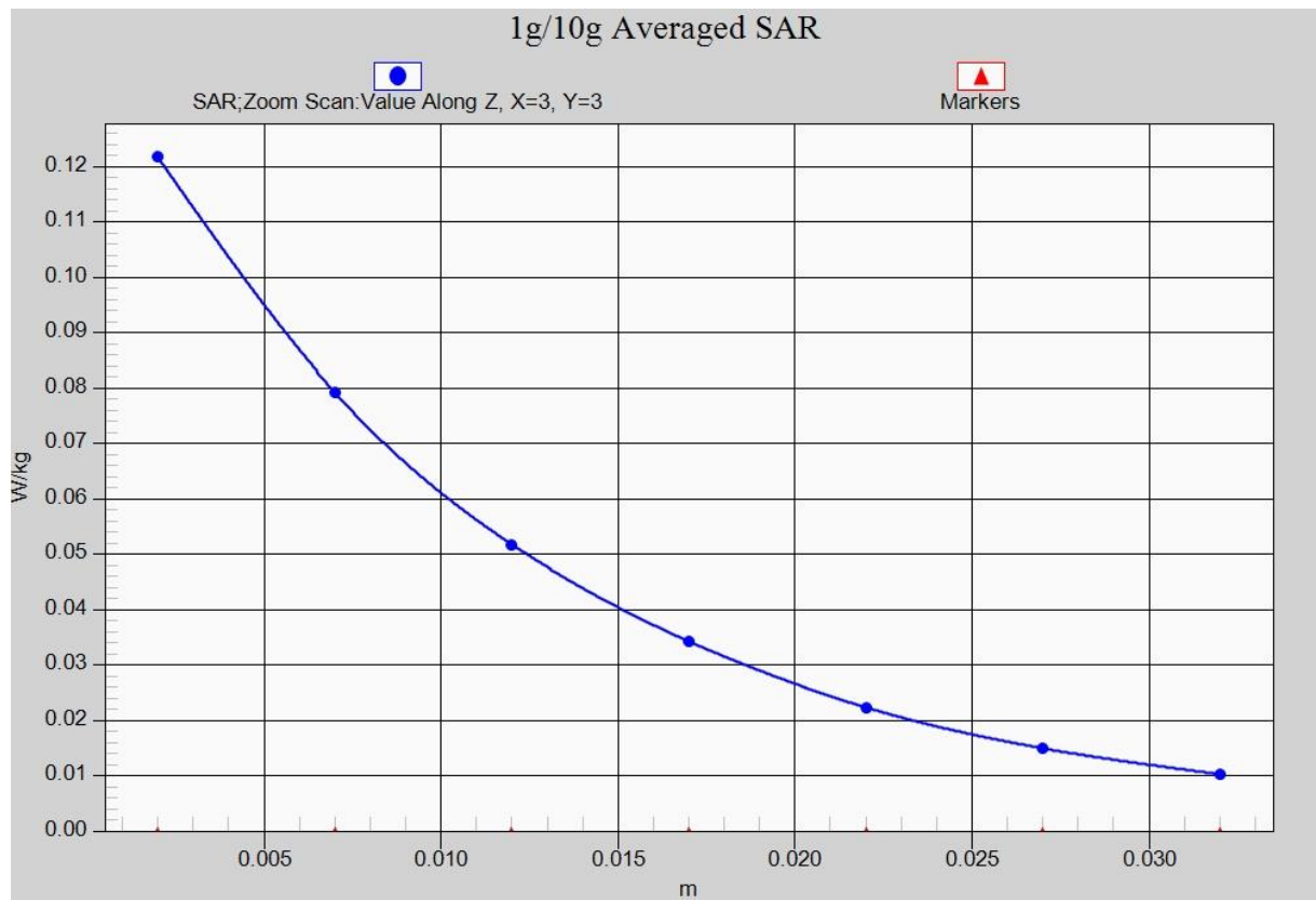
Fig. 3-1 Z-Scan at power reference point (GSM1900)
