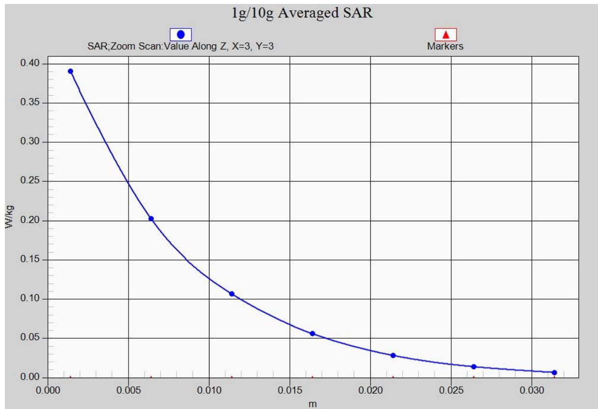
Fig. 12-1 Z-Scan at power reference point (LTE Band 41)
