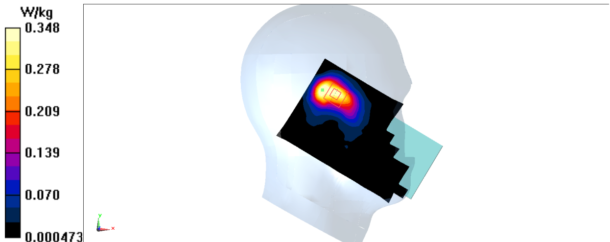
Fig.13 Wifi 802.11b
