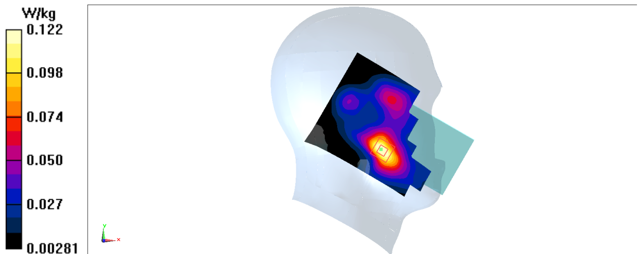
Fig.3 GSM1900
