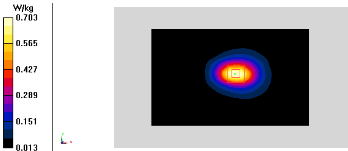
Fig.4 GSM1900
