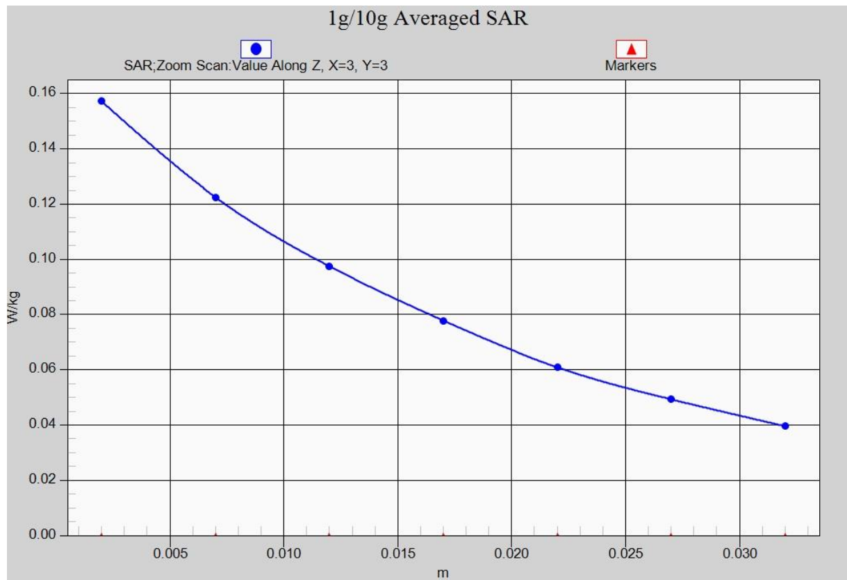
Fig. 1-1 Z-Scan at power reference point (GSM850)
