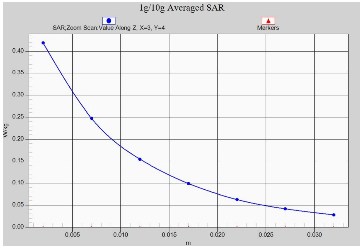
Fig. 2-1 Z-Scan at power reference point (GSM850)
