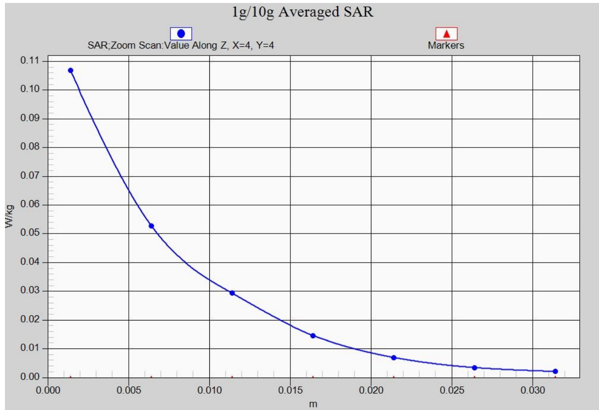
Fig. 14-1 Z-Scan at power reference point (Wifi 802.11b)
