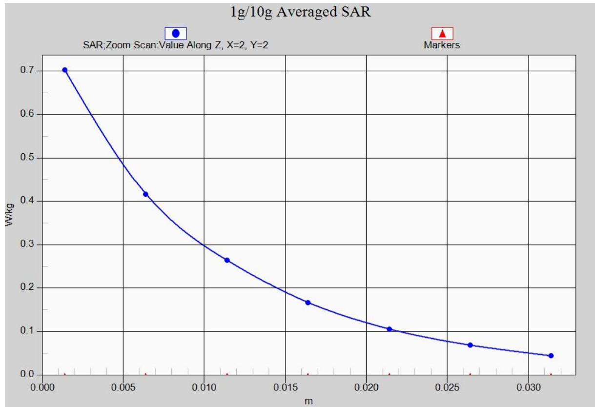
Fig. 4-1 Z-Scan at power reference point (GSM1900)
