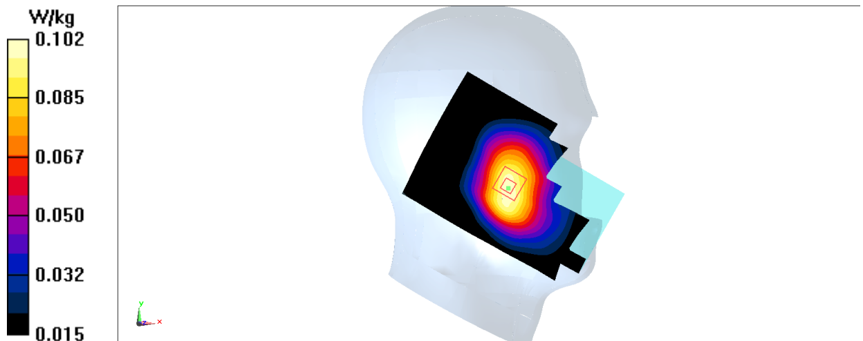
Fig.7 LTE Band5
