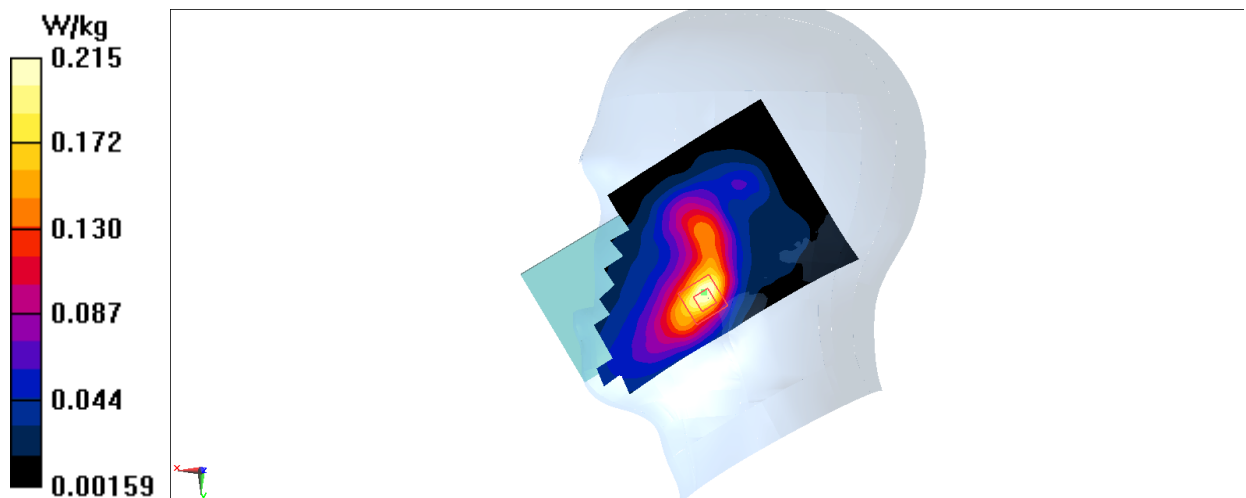
Fig.11 LTE Band 41
