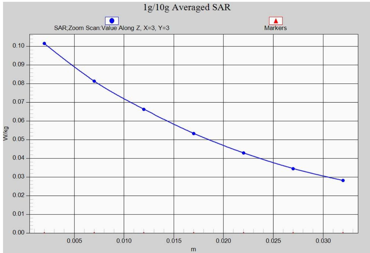
Fig. 7-1 Z-Scan at power reference point (LTE Band5)
