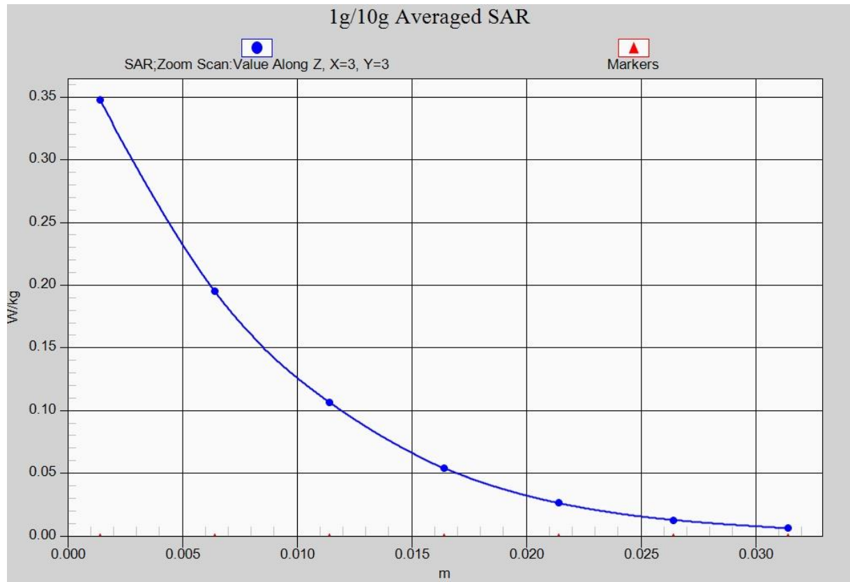
Fig. 13-1 Z-Scan at power reference point (Wifi 802.11b)
