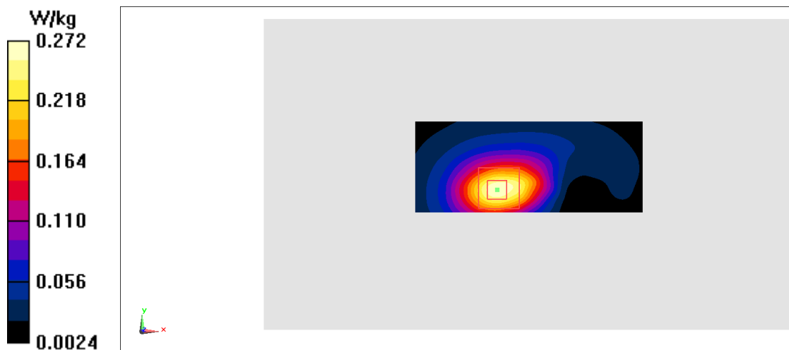
Fig.12 LTE Band 41
