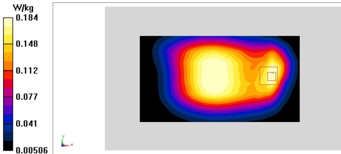
Fig.8 LTE Band5
