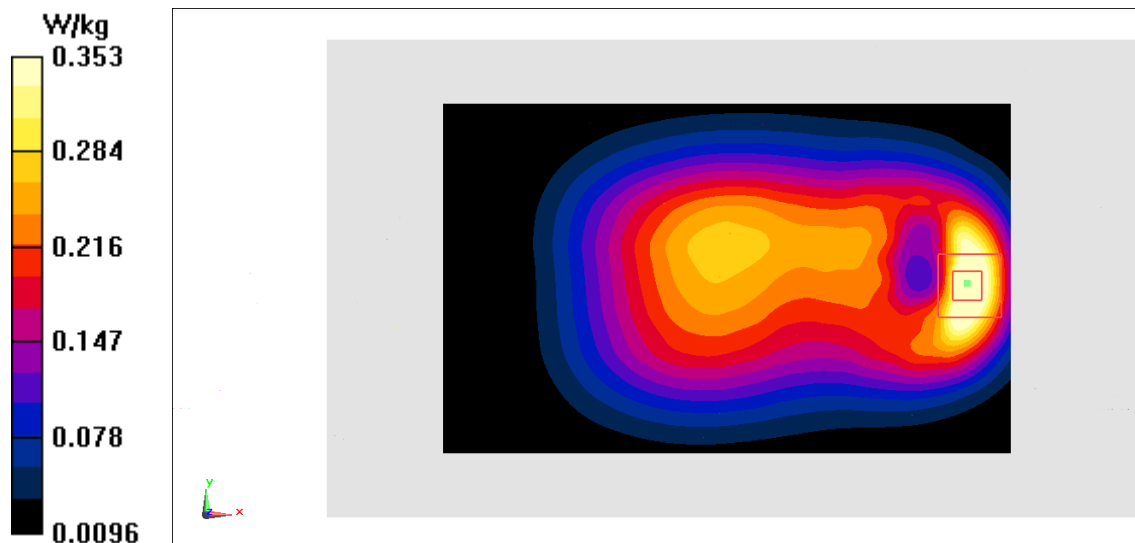
Fig.2 GSM850
