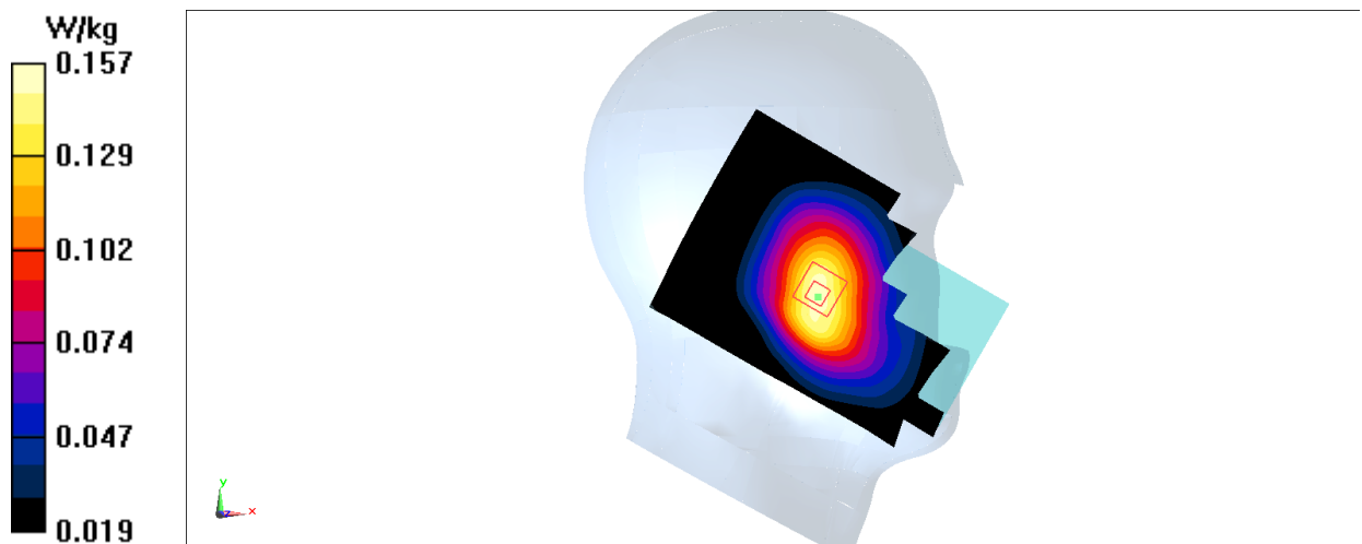
Fig.1 GSM850
