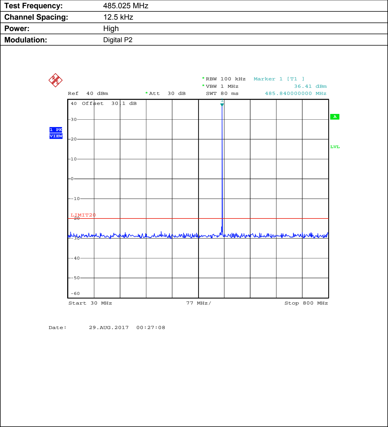
Plot 5.9.4.2.1. Conducted Transmitter Spurious Emissions for 485.025 MHz, High Power
