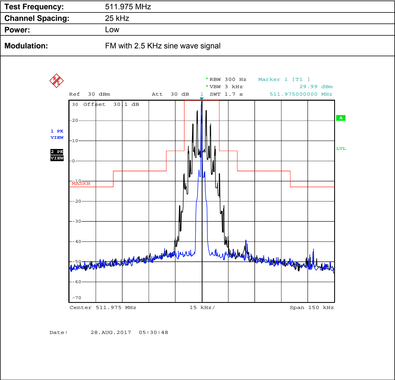
Plot 5.8.4.3.6. Emission Mask B, Low Power
