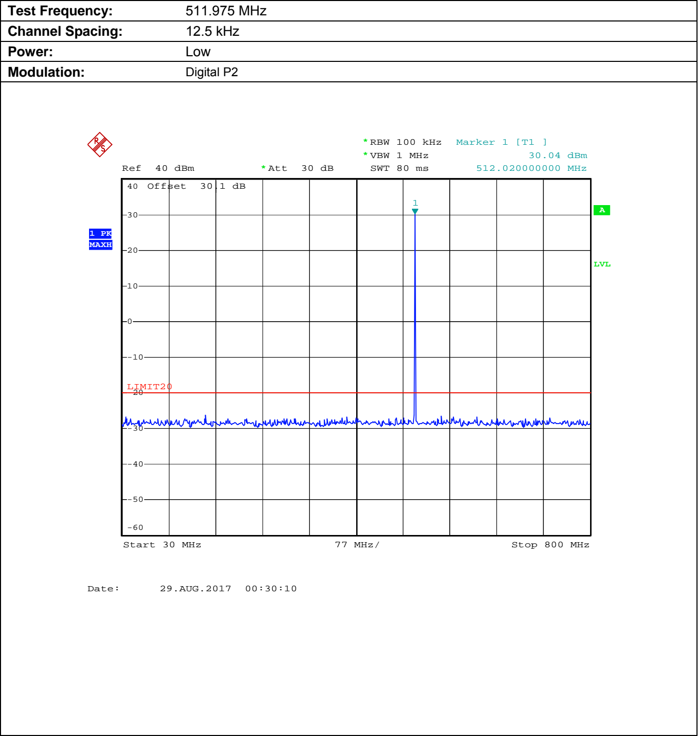
Plot 5.9.4.3.2. Conducted Transmitter Spurious Emissions for 511.975 MHz, Low Power
