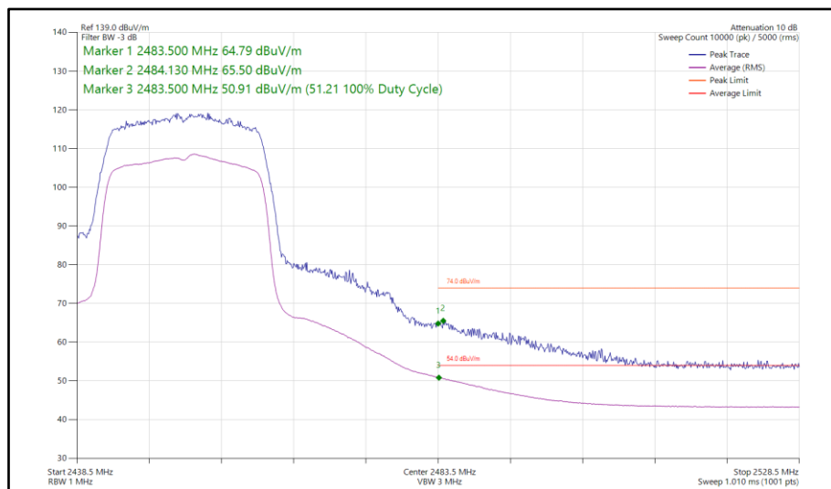
Figure 39 - 802.11ax HE20, SU, SISO, Core 0 - 2452 MHz Band Edge Frequency 2483.5 MHz
