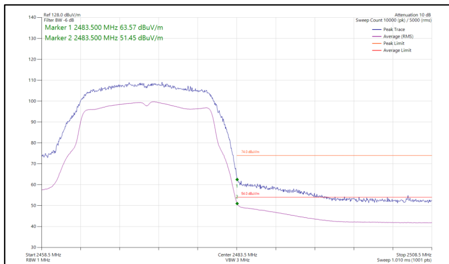
Figure 29 - 802.11g, SISO, Core 0 - 2472 MHz Band Edge Frequency 2483.5 MHz
