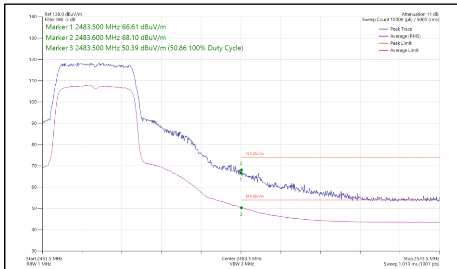
Figure 38 - 802.11ax HE20, SU, SISO, Core 0 - 2447 MHz Band Edge Frequency 2483.5 MHz
