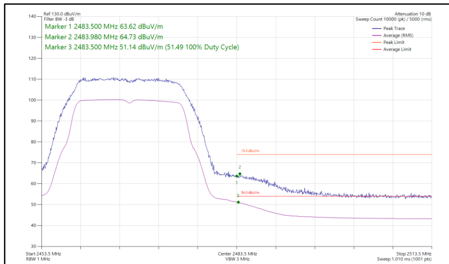
Figure 28 - 802.11g, SISO, Core 0 - 2467 MHz Band Edge Frequency 2483.5 MHz
