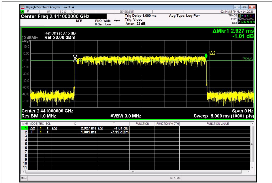
(3DH5_2441M, 8-DQPSK)
