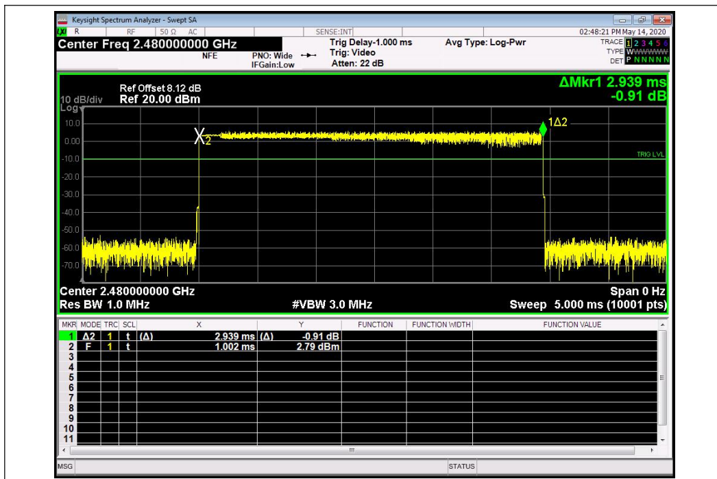
(3DH5_2480M, 8-DQPSK)
