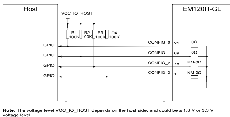
Figure 31: Recommended Circuit of EM120R-GL Configuration Pins
