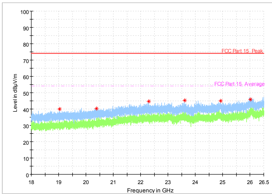
Fig. 39 Radiated Spurious Emission (802.11a, ch40, 18 GHz-26.5 GHz)
