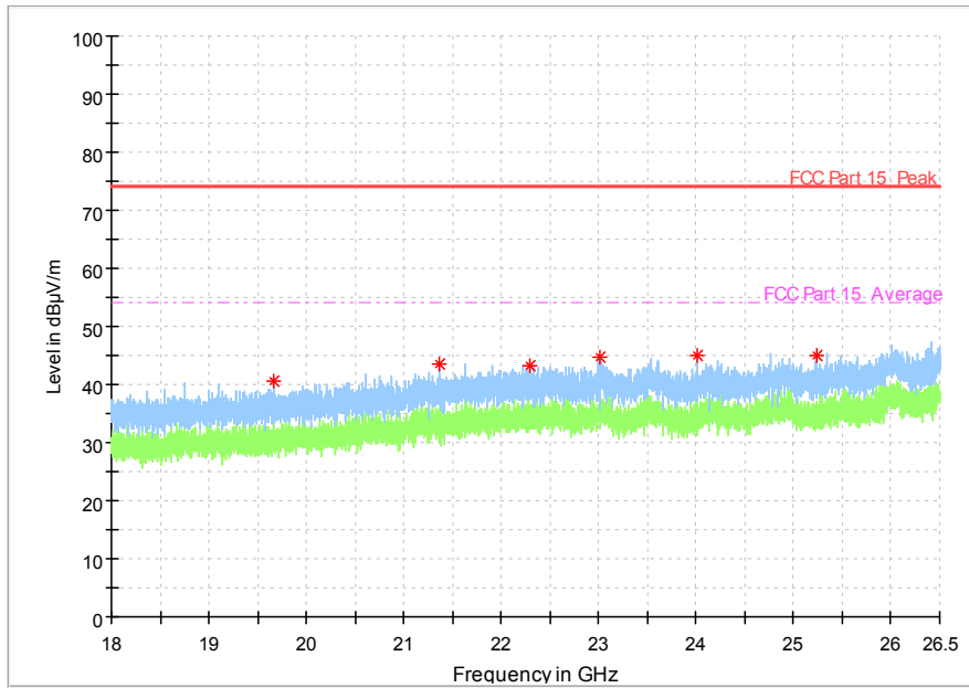
Fig. 44 Radiated Spurious Emission (802.11a, ch48, 18 GHz-26.5 GHz)
