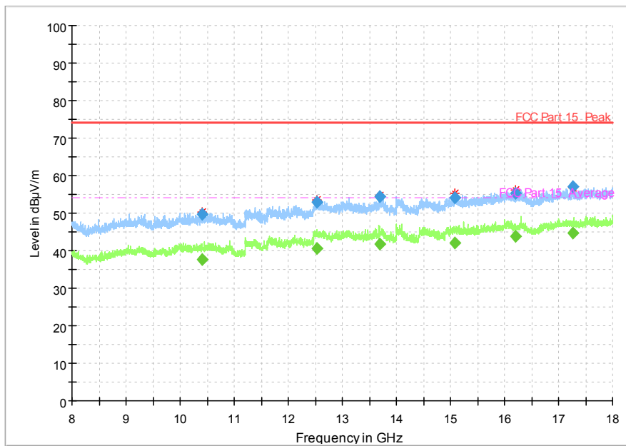
Fig. 63 Radiated Spurious Emission (802.11 n-HT40, ch38, 8 GHz-18 GHz)
