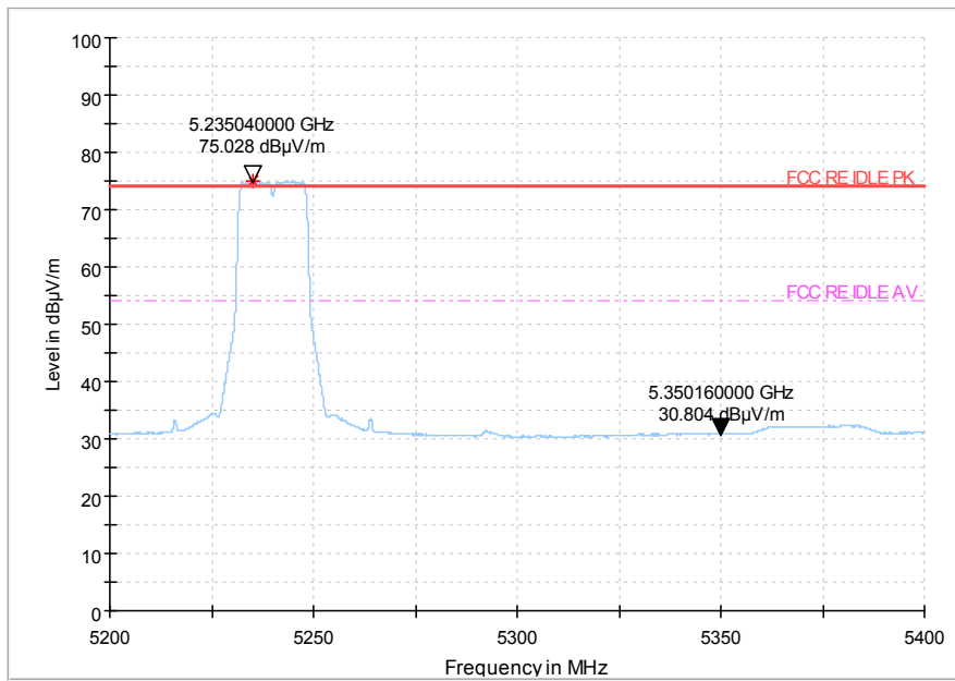
Fig. 24 Band Edges (802.11a, 5240MHz)
