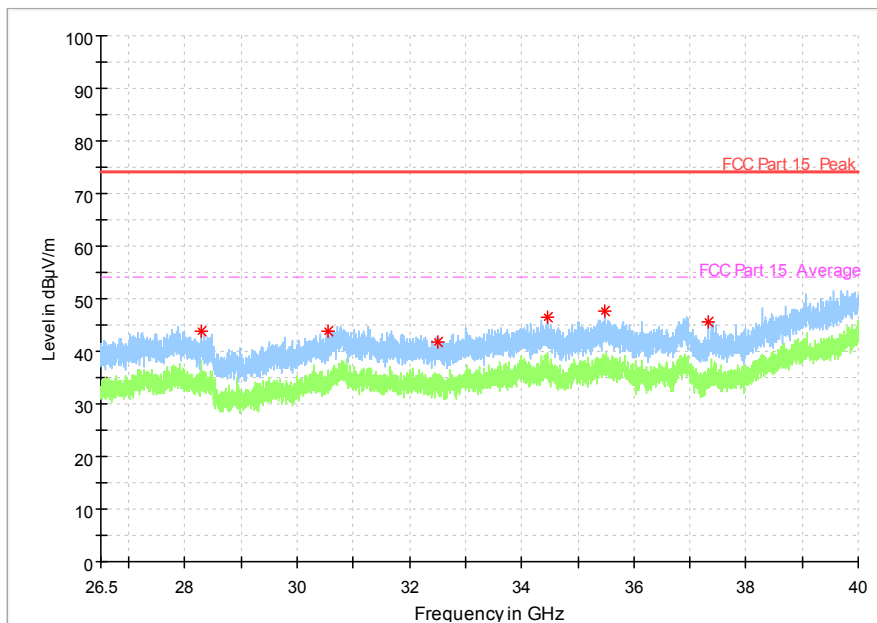
Fig. 45 Radiated Spurious Emission (802.11a, ch48, 26.5 GHz-40 GHz)
