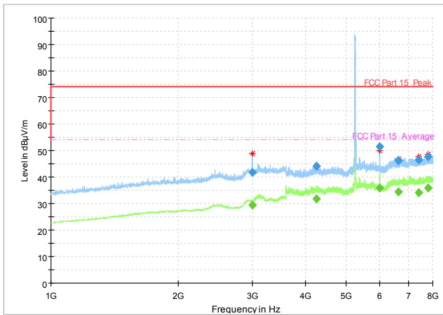
Fig. 57 Radiated Spurious Emission (802.11 n-HT20, ch48, 1 GHz-8 GHz)
