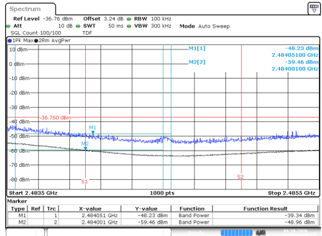
BE-R-HIGH-2MHz, MIMO-B, 802.11ax40-HE0, Ch13
