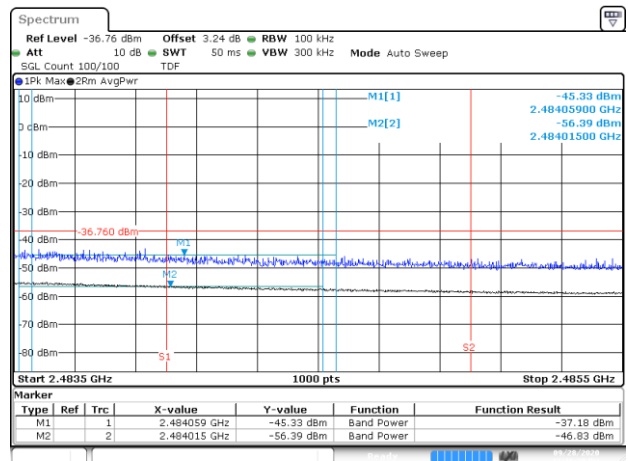
BE-R-HIGH-2MHz, MIMO-B, 802.11ax40-HE0, Ch12
