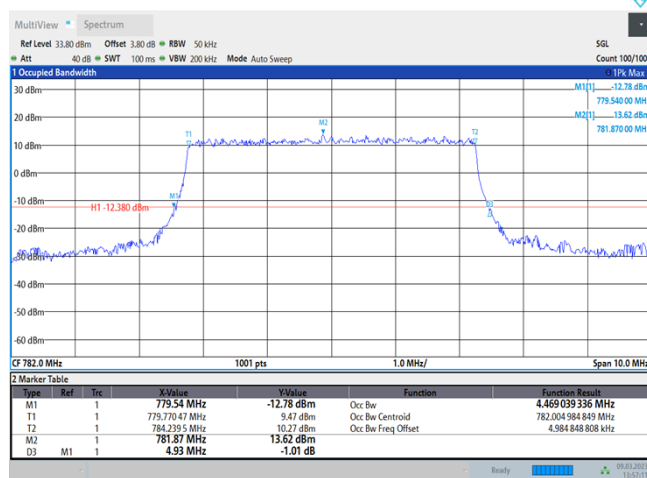
Band13-5MHz-QPSK-23230-25RB#0
