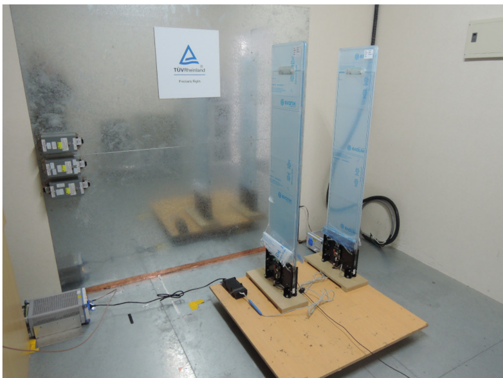
Photograph 5: Set-up for Mains Conducted testing Front
