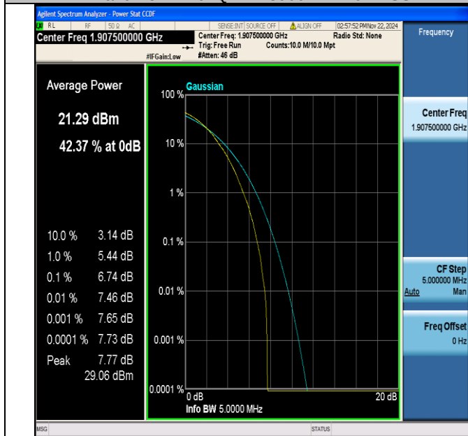
Band2-5MHz-64QAM-19175-1RB#0-PASS
