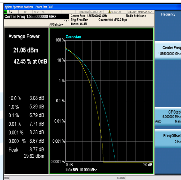
Band2-10MHz-64QAM-18650-50RB#0-PASS
