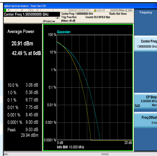
Band2-10MHz-64QAM-19150-50RB#0-PASS
