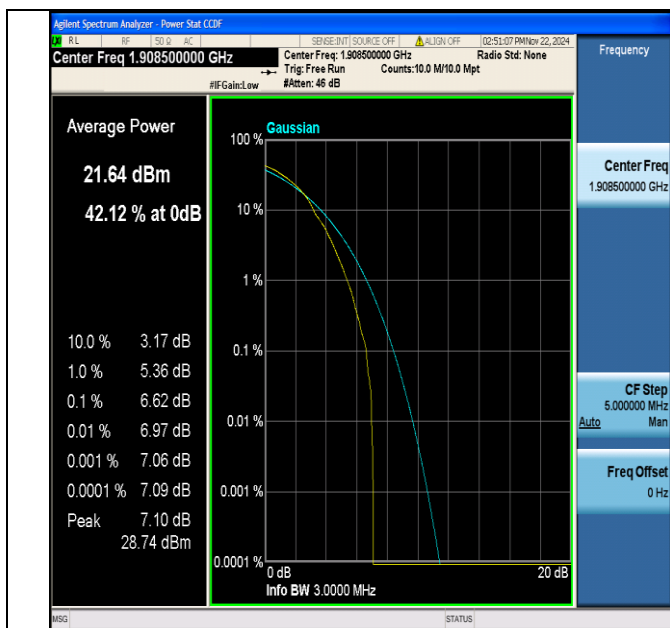
Band2-3MHz-64QAM-19185-1RB#0-PASS
