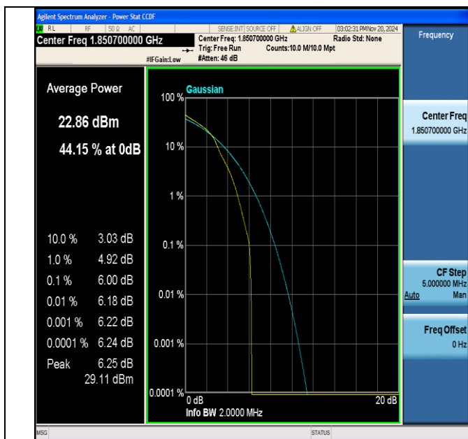
Band2-1.4MHz-16QAM-18607-1RB#0-PASS
