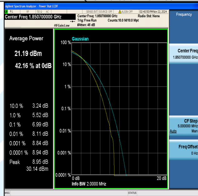
Band2-1.4MHz-64QAM-18607-6RB#0-PASS
