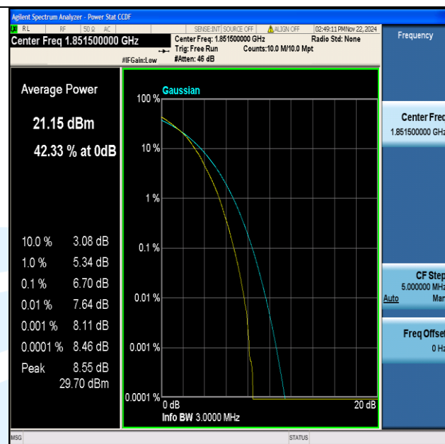
Band2-3MHz-64QAM-18615-15RB#0-PASS
