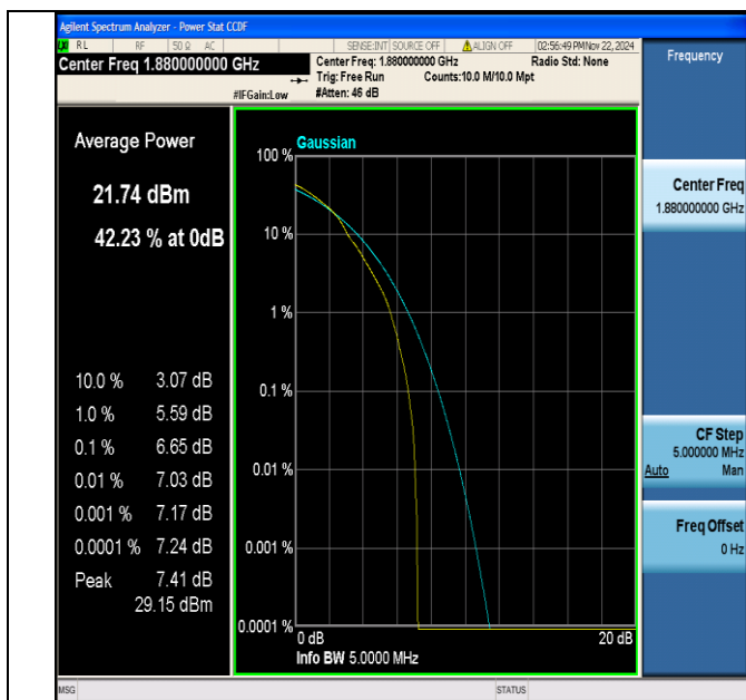
Band2-5MHz-64QAM-18900-1RB#0-PASS
