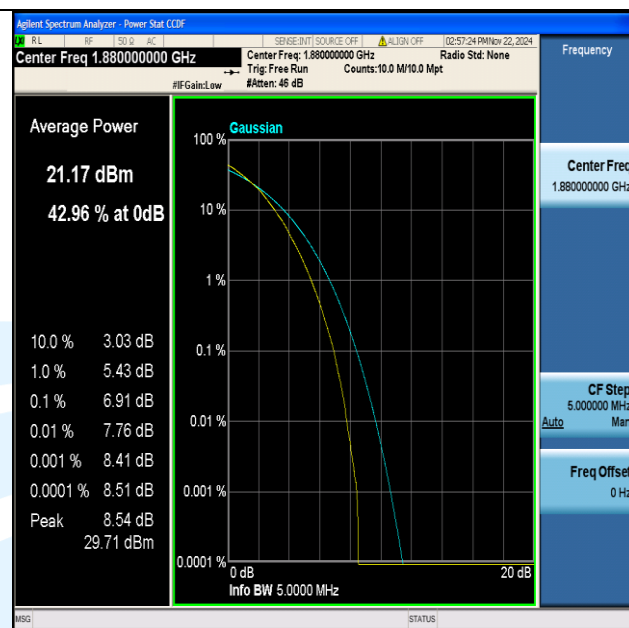
Band2-5MHz-64QAM-18900-25RB#0-PASS
