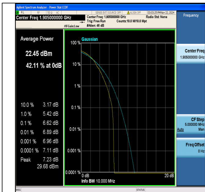
Band2-10MHz-64QAM-19150-1RB#0-PASS
