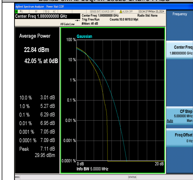
Band2-5MHz-16QAM-18900-1RB#0-PASS
