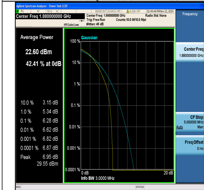
Band2-3MHz-64QAM-18900-1RB#0-PASS
