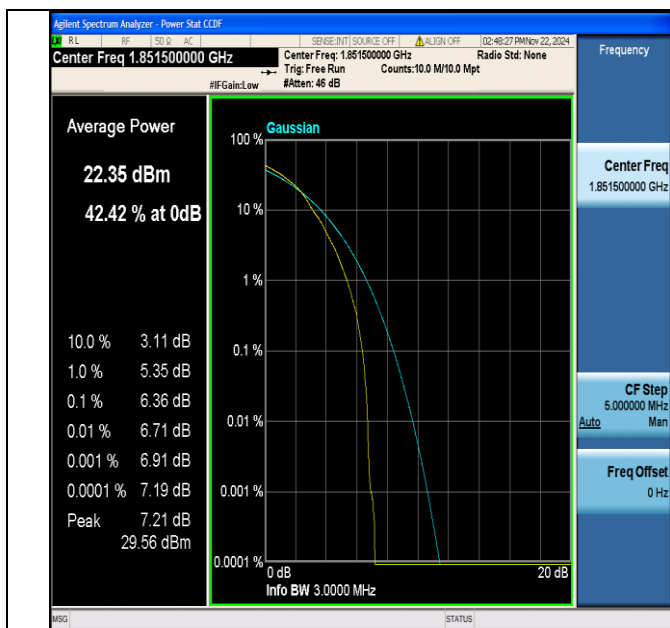
Band2-3MHz-64QAM-18615-1RB#0-PASS
