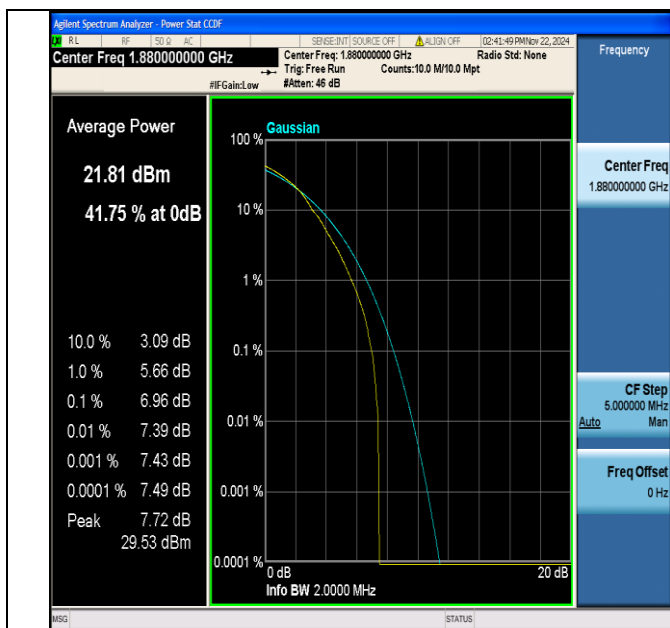
Band2-1.4MHz-64QAM-18900-1RB#0-PASS
