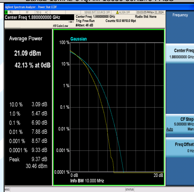
Band2-10MHz-64QAM-18900-50RB#0-PASS
