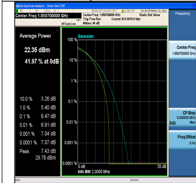
Band2-1.4MHz-64QAM-18607-1RB#0-PASS
