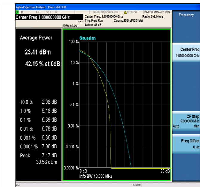
Band2-10MHz-16QAM-18900-1RB#0-PASS
