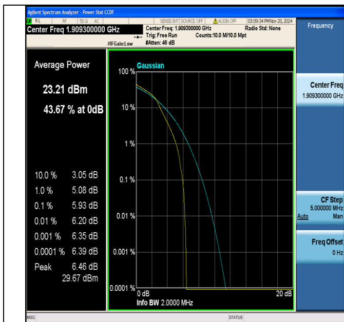
Band2-1.4MHz-16QAM-19193-1RB#0-PASS
