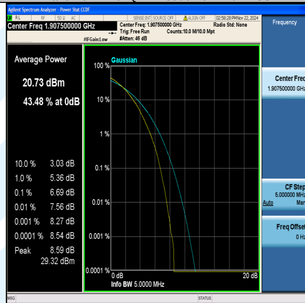
Band2-5MHz-64QAM-19175-25RB#0-PASS
