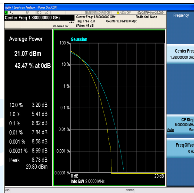
Band2-1.4MHz-64QAM-18900-6RB#0-PASS
