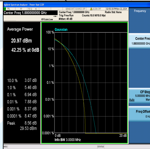
Band2-3MHz-64QAM-18900-15RB#0-PASS
