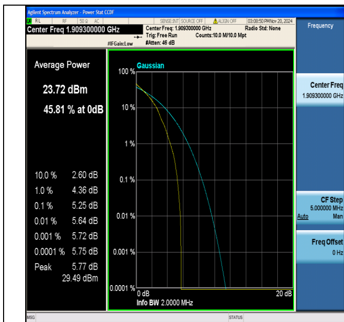
Band2-1.4MHz-QPSK-19193-1RB#0-PASS
