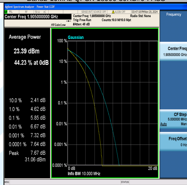
Band2-10MHz-QPSK-19150-50RB#0-PASS
