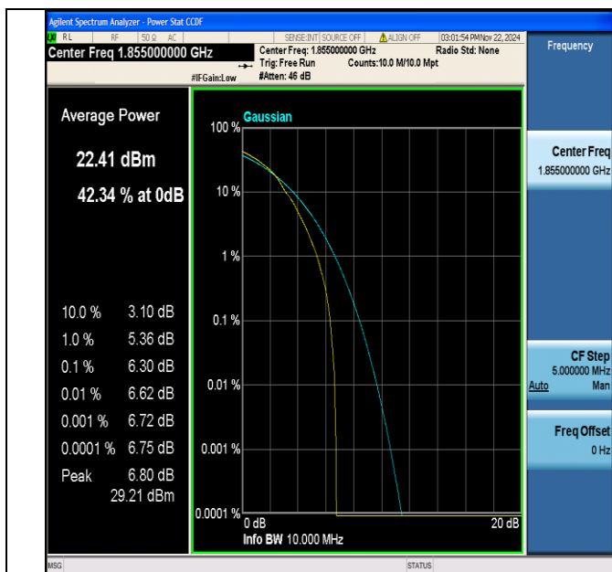
Band2-10MHz-64QAM-18650-1RB#0-PASS
