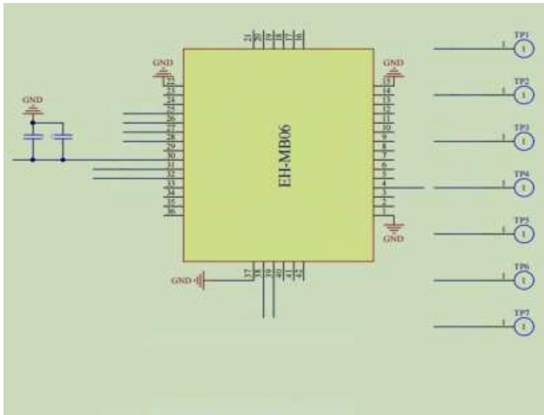
Figure 13: Reference Design
