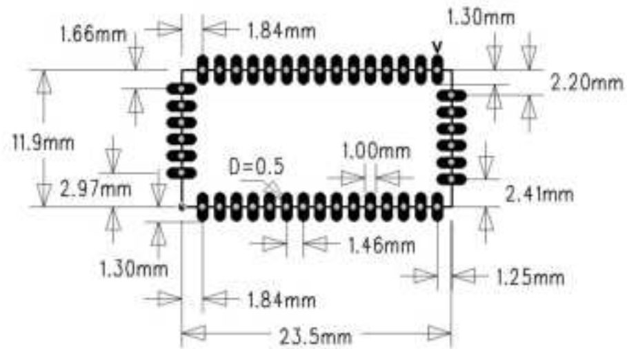
Figure 15: Recommended PCB Mounting Pattern (Unit: mm, Deviation:0.02mm)
