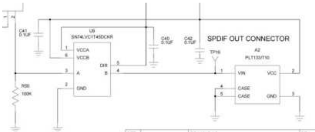
Figure 9: Example Circuit for SPDIF Out Connector
