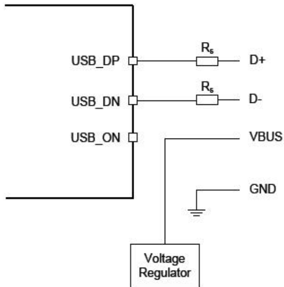
Figure 12: USB Connections
