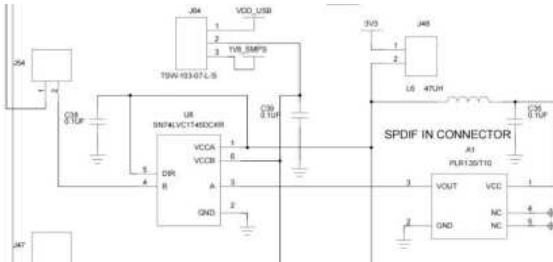
Figure 8: Example Circuit for SPDIF In Connector
