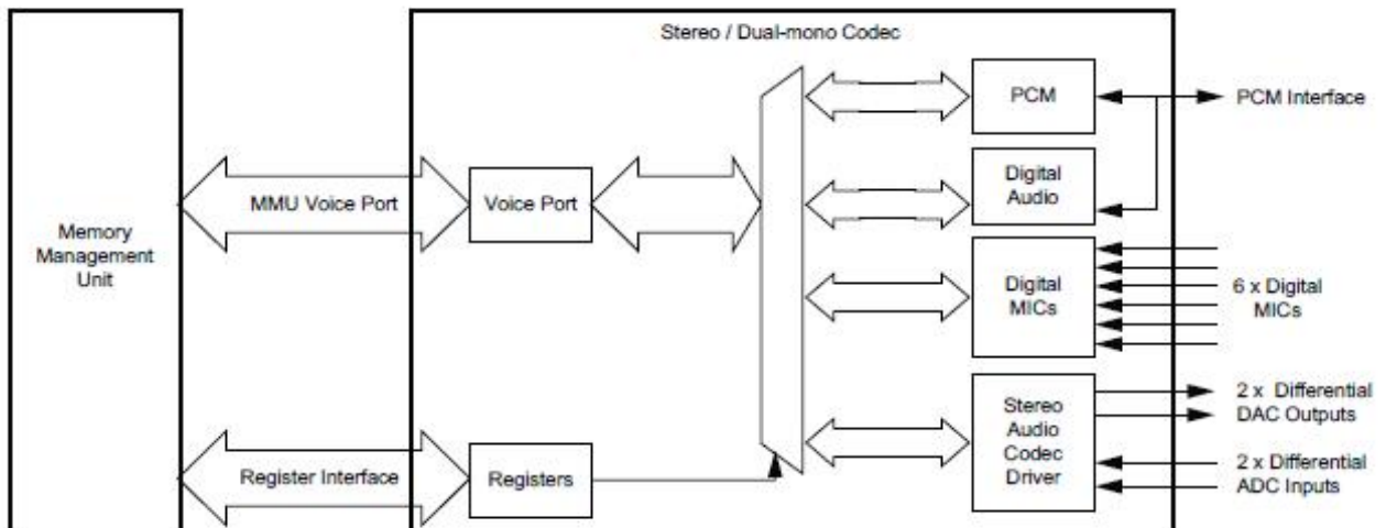
Figure 4 : Audio Interface
