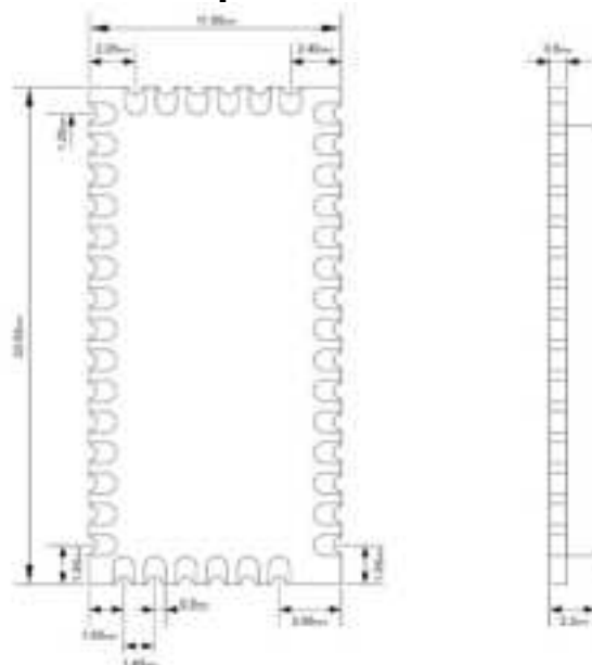
Figure 14: Mechanical Drawing
