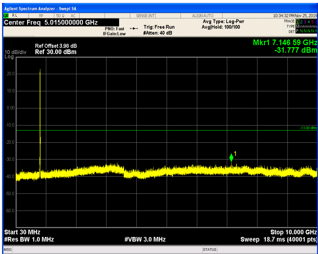
LTE Band19 QPSK BW=5MHz Channel=24125 RB Size=25 Position=#0
