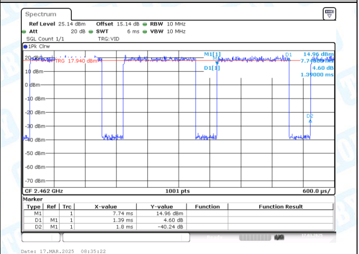
NTNV-11G-Ant1-2462
