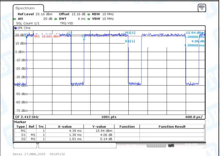
NTNV-11G-Ant1-2412
