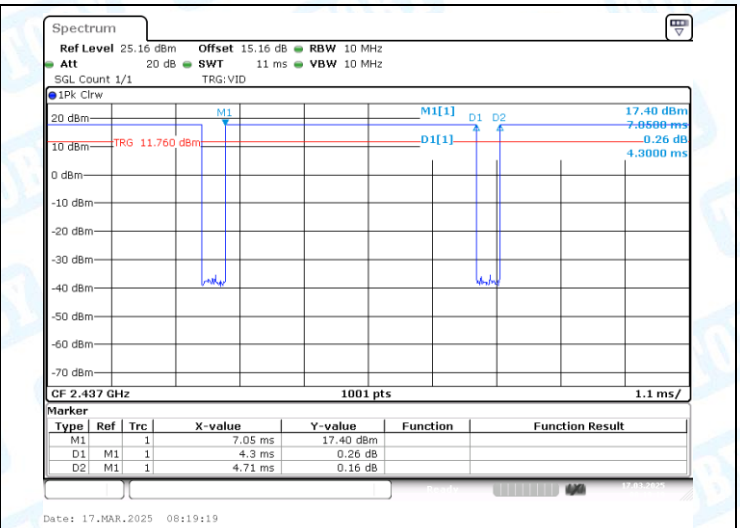
NTNV-11B-Ant1-2437
