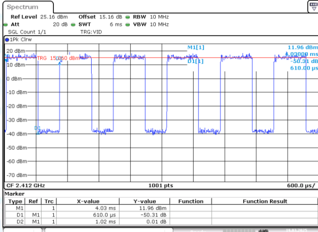
NTNV-11N20MIMO-Ant1-2412
