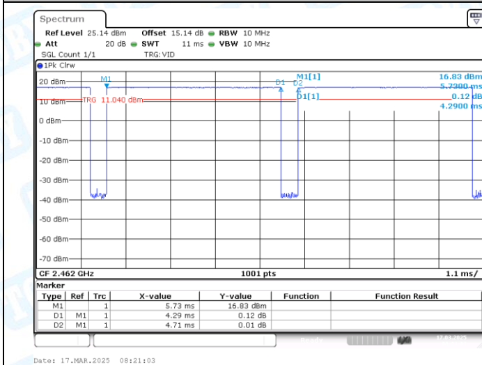
NTNV-11B-Ant1-2462
