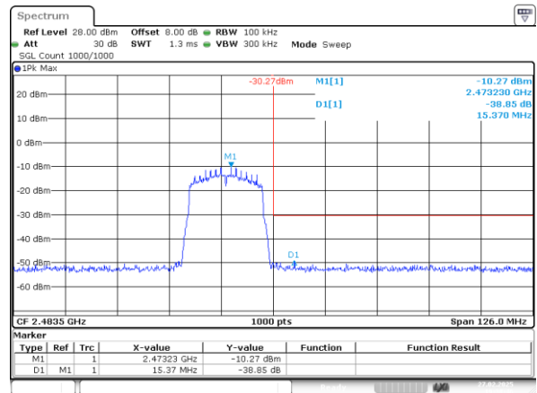
802.11n20_2472MHz_Chain 1
