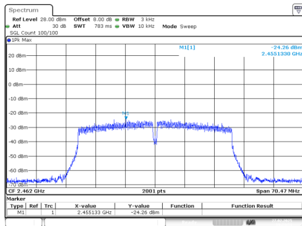
802.11n40_2462MHz_Chain 0
