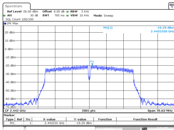
802.11n40_2442MHz_Chain 1
