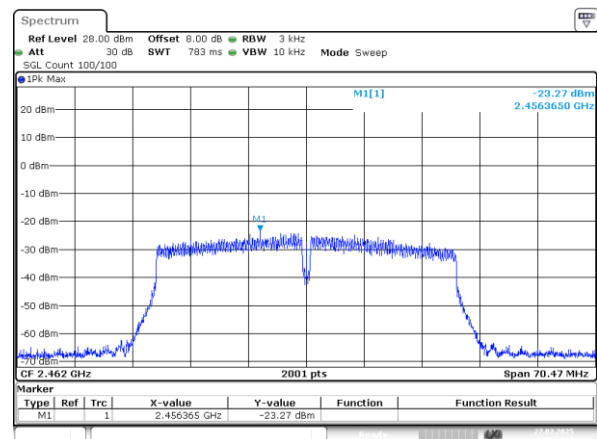
802.11n40_2462MHz_Chain 1
