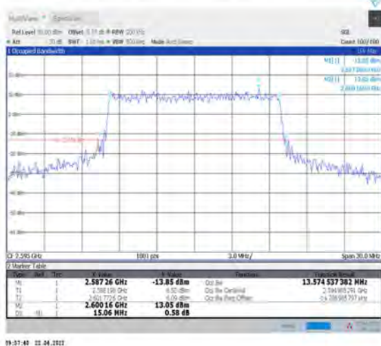
1-N38--30-15-M-7-CP-16QAM-Outer_Full-38@0-Ant1-13.575-15.060-≤15-PASS
