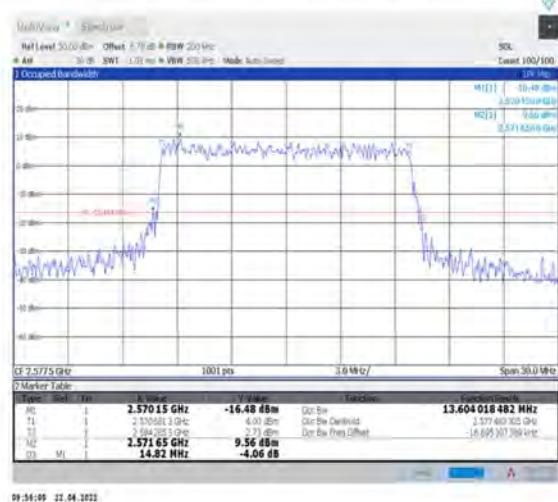
1-N38--30-15-L-9-CP-256QAM-Outer_Full-38@0-Ant1-13.604-14.820-≤15-PASS
