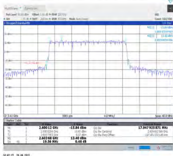
1-N38--30-20-H-3-DFT-16QAM-Outer_Full-50@0-Ant1-17.948-19.560-≤20-PASS
