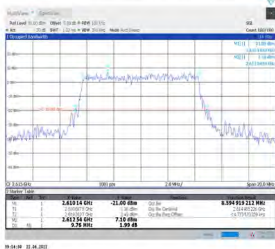
1-N38--30-10-H-9-CP-256QAM-Outer_Full-24@0- Ant1-8.595-9.760-≤10-PASS
