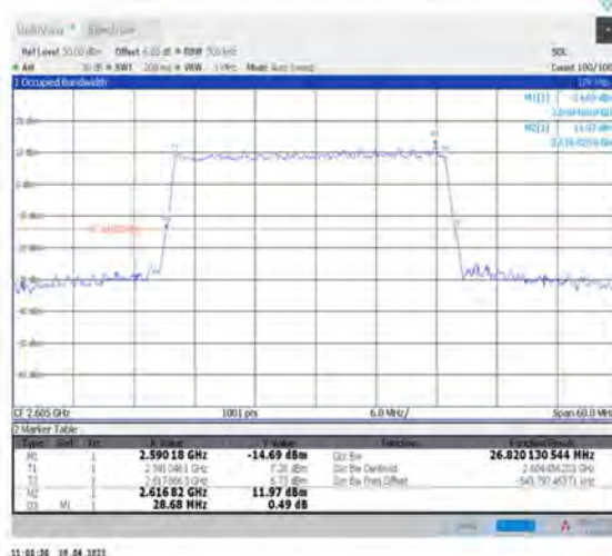
1-N38--30-30-H-5-DFT-256QAM-Outer_Full-75@0-Ant1-26.82-28.680-≤30-PASS
