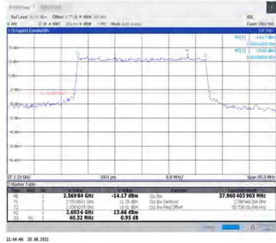
1-N38--30-40-L-6-CP-QPSK-Outer_Full-106@0-Ant1-37.96-40.320-≤40-PASS
