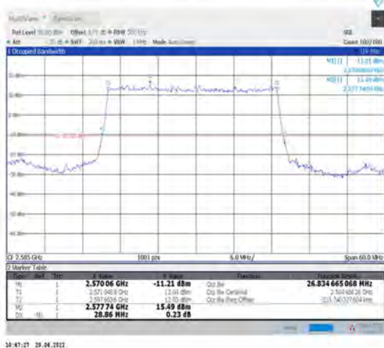
1-N38--30-30-L-2-DFT-PI2BPSK-Outer_Full-75@0-Ant1-26.835-28.860-≤30-PASS
