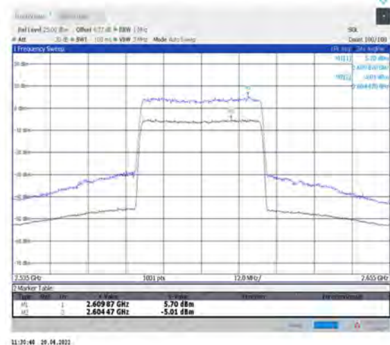
1-N38--30-40-M-2-CP-256QAM-Outer_Full-106@0- Ant1-10.71-19.4%-7.12-3.59-PASS-≤13
