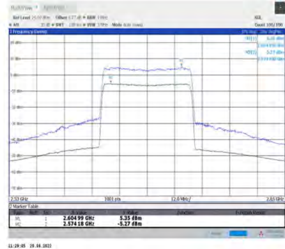
1-N38--30-40-L-2-CP-256QAM-Outer_Full-106@0- Ant1-10.62-19.4%-7.12-3.50-PASS-≤13
