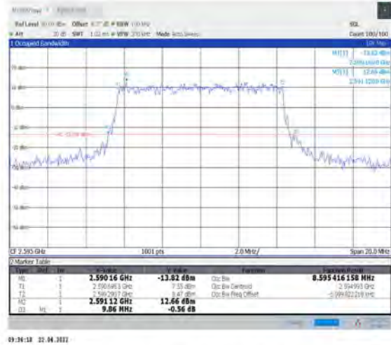
1-N38--30-10-M-1-DFT-QPSK-Outer_Full-24@0-Ant1-8.595-9.860-≤10-PASS
