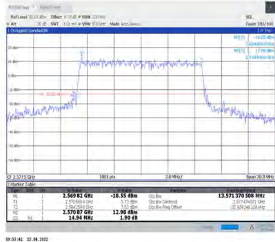
1-N38--30-15-L-7-CP-16QAM-Outer_Full-38@0-Ant1-13.571-14.940-≤15-PASS
