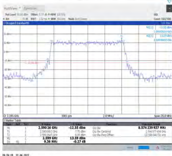
1-N38--30-10-M-2-DFT-PI2BPSK-Outer_Full-24@0-Ant1-8.574-9.360-≤10-PASS
