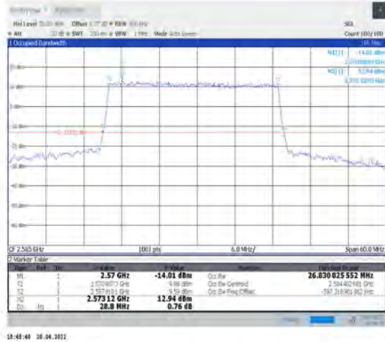
1-N38--30-30-L-4-DFT-64QAM-Outer_Full-75@0- Ant1-26.831-28.800-≤30-PASS
