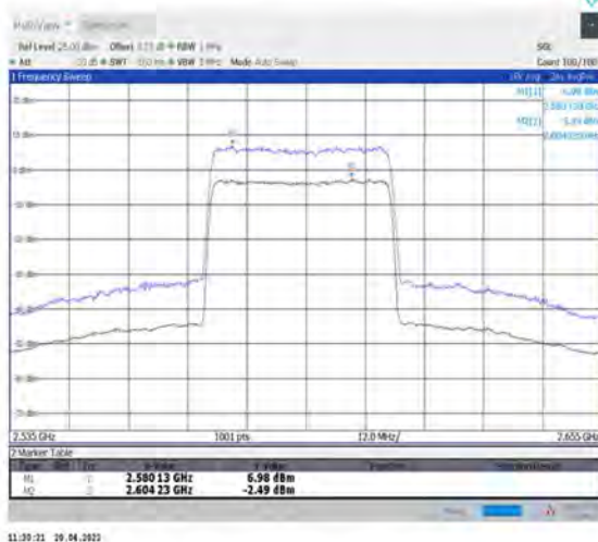
1-N38--30-40-M-1-DFT-256QAM-Outer_Full-100@0- Ant1-9.47-19.4%-7.12-2.35-PASS-≤13
