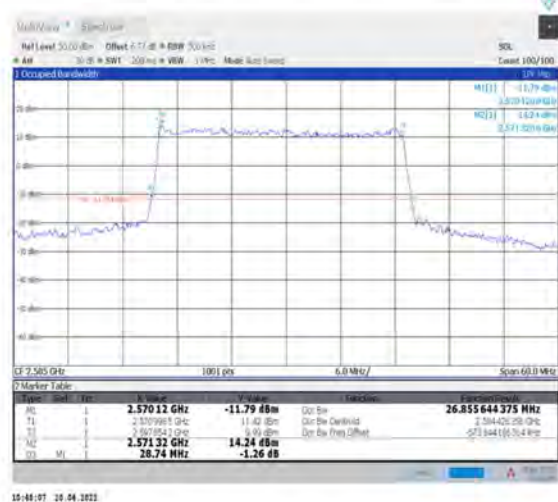
1-N38--30-30-L-3-DFT-16QAM-Outer_Full-75@0-Ant1-26.856-28.740-≤30-PASS
