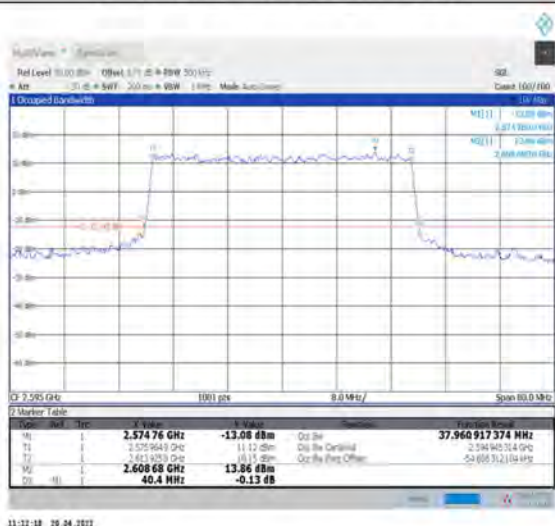
1-N38--30-40-M-6-CP-QPSK-Outer_Full-106@0-Ant1-37.961-40.400-≤40-PASS
