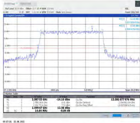
1-N38--30-15-M-6-CP-QPSK-Outer_Full-38@0-Ant1-13.581-14.640-≤15-PASS
