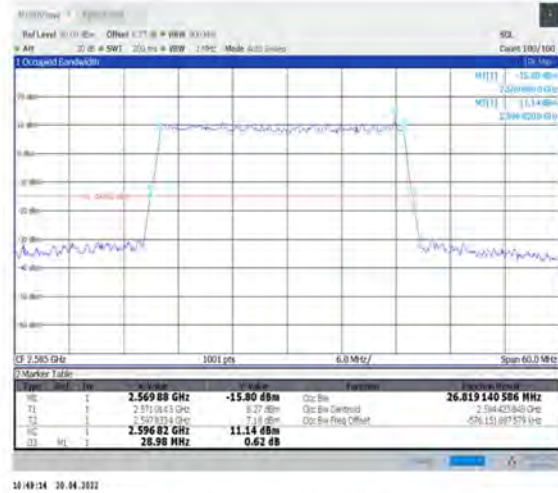
1-N38--30-30-L-5-DFT-256QAM-Outer_Full-75@0- Ant1-26.819-28.980-≤30-PASS
