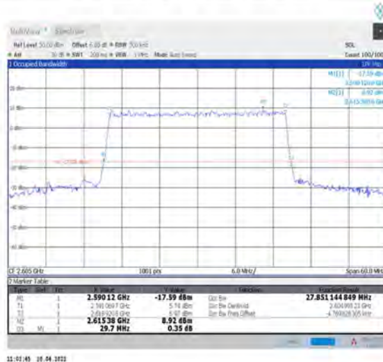
1-N38--30-30-H-9-CP-256QAM-Outer_Full-78@0-Ant1- 27.851-29.700-≤30-PASS
