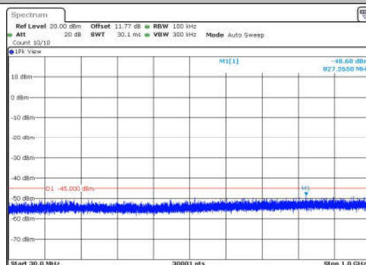
11N20SISO-Ant1-2412-30~1000-PASS
