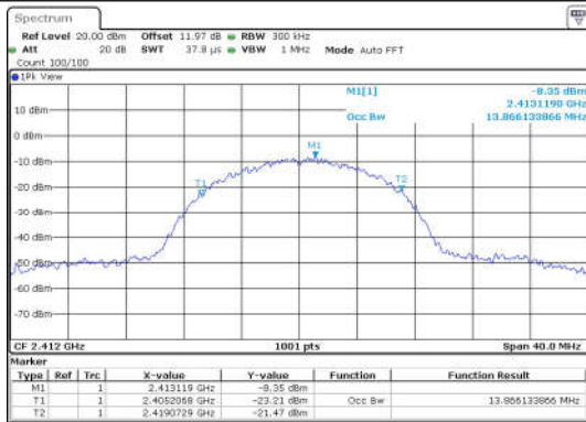
11B-Ant1-2412
