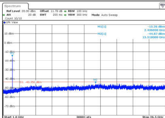
11G-Ant1-2437-1000~26500-PASS
