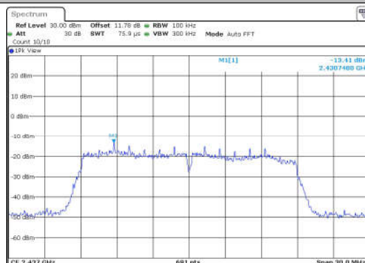
11N20SISO-Ant1-2437-0~Reference-PASS
