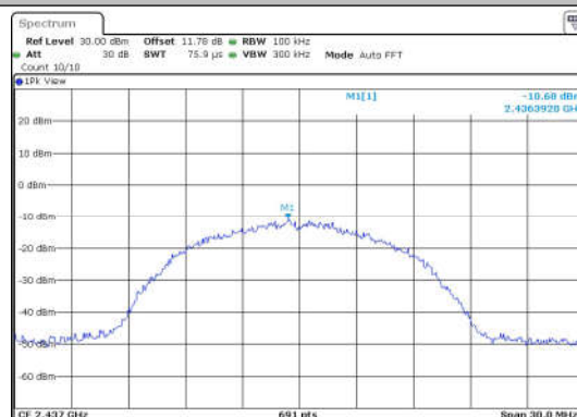
11B-Ant1-2437-0~Reference-PASS
