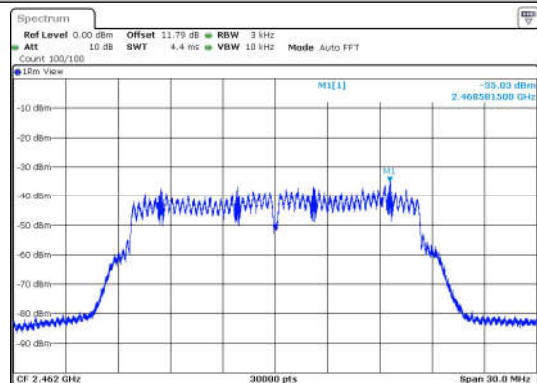
11G-Ant1-2462-PASS
