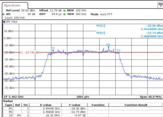
11N20SISO-Ant1-2462-PASS
