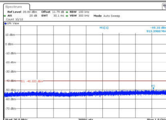
11B-Ant1-2462-30~1000-PASS
