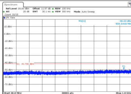
11B-Ant1-2412-30~1000-PASS
