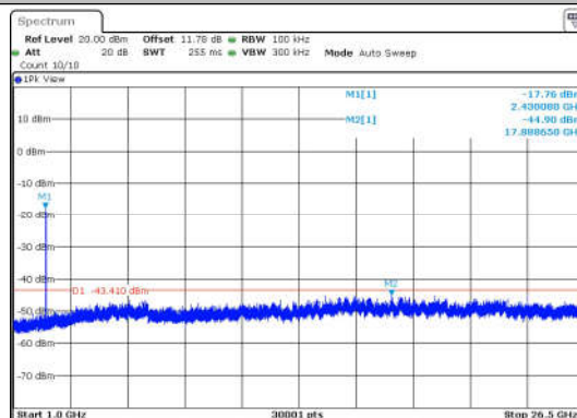
11N20SISO-Ant1-2437-1000~26500-PASS
