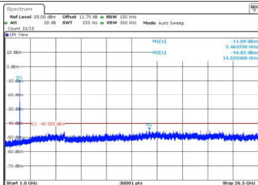
11B-Ant1-2462-1000~26500-PASS
