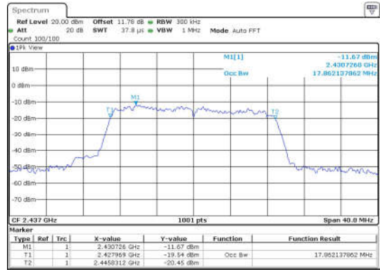
11N20SISO-Ant1-2437
