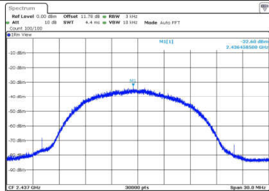
11B-Ant1-2437-PASS
