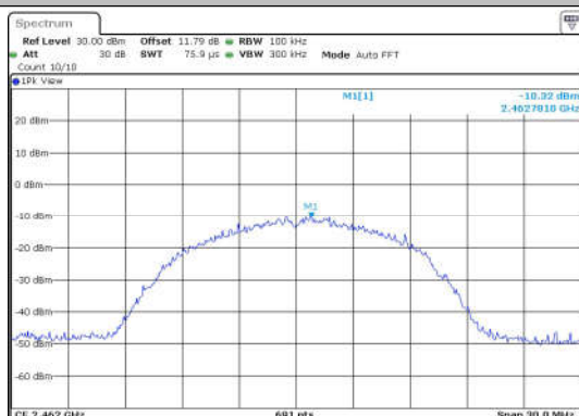
11B-Ant1-2462-0~Reference-PASS
