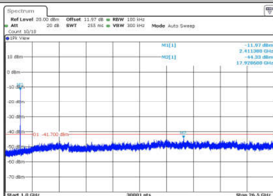
11B-Ant1-2412-1000~26500-PASS
