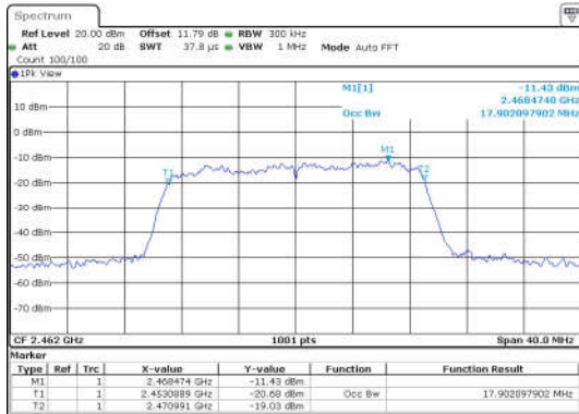
11N20SISO-Ant1-2462
