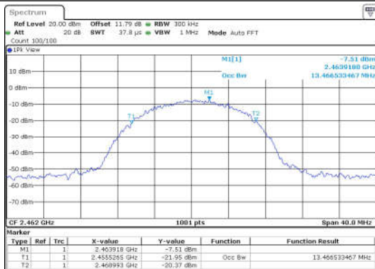
11B-Ant1-2462
