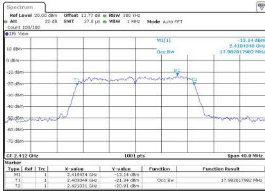
11N20SISO-Ant1-2412
