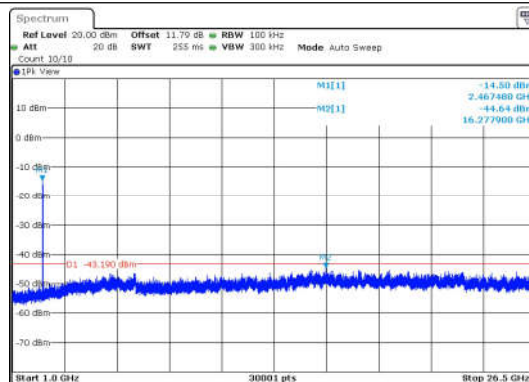
11G-Ant1-2462-1000~26500-PASS
