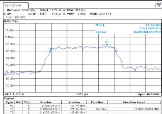
11G-Ant1-2412
