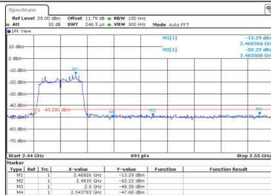
11N20SISO-Ant1-2462-PASS
