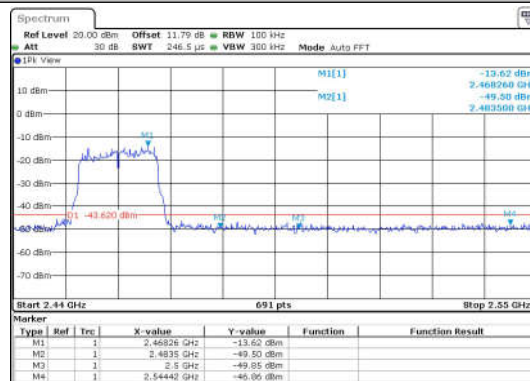
11G-Ant1-2462-PASS
