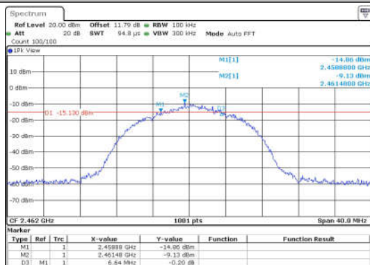
11B-Ant1-2462-PASS
