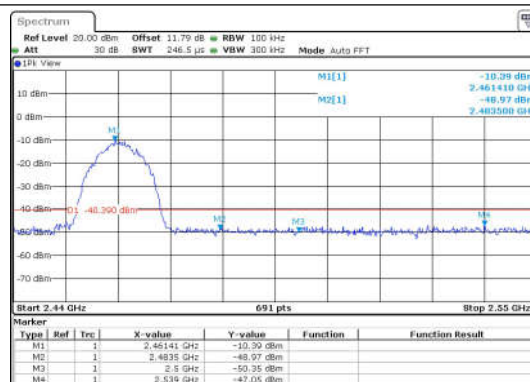
11B-Ant1-2462-PASS
