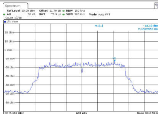
11G-Ant1-2462-0~Reference-PASS
