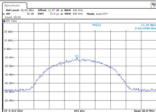
11B-Ant1-2412-0~Reference-PASS
