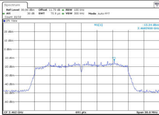
11N20SISO-Ant1-2462-0~Reference-PASS
