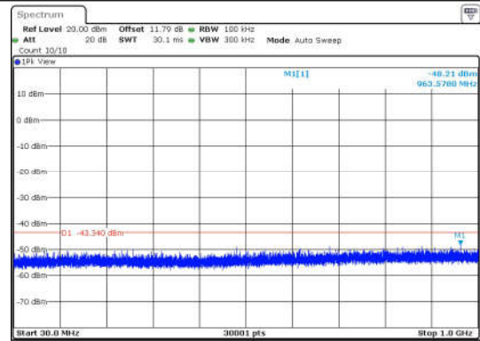
11N20SISO-Ant1-2462-30~1000-PASS
