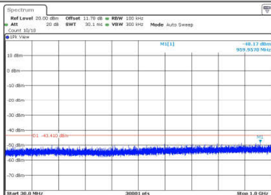
11N20SISO-Ant1-2437-30~1000-PASS
