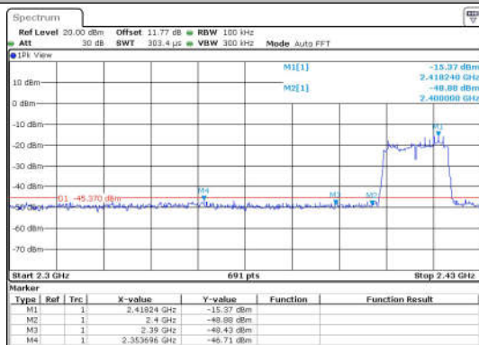
11N20SISO-Ant1-2412-PASS
