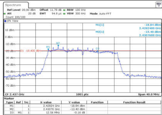
11N20SISO-Ant1-2437-PASS
