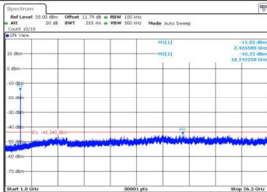
11N20SISO-Ant1-2462-1000~26500-PASS
