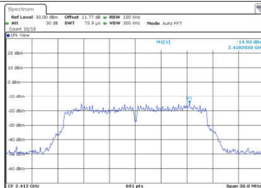
11G-Ant1-2412-0~Reference-PASS
