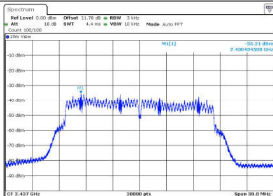
11G-Ant1-2437-PASS
