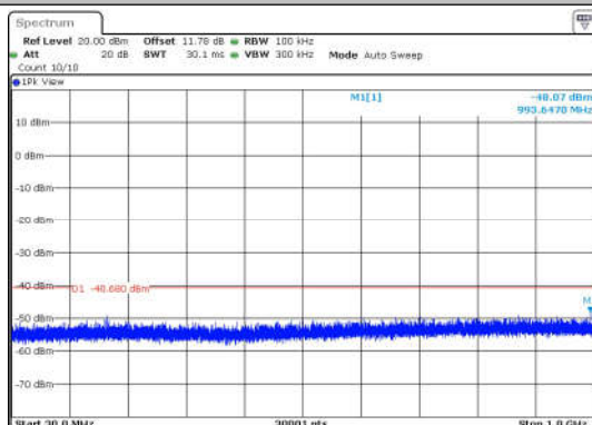
11B-Ant1-2437-30~1000-PASS
