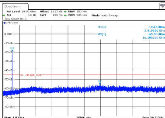
11N20SISO-Ant1-2412-1000~26500-PASS
