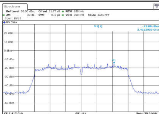
11N20SISO-Ant1-2412-0~Reference-PASS
