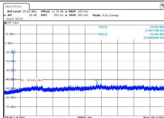
11B-Ant1-2437-1000~26500-PASS
