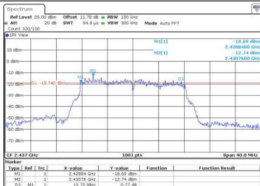
11G-Ant1-2437-PASS
