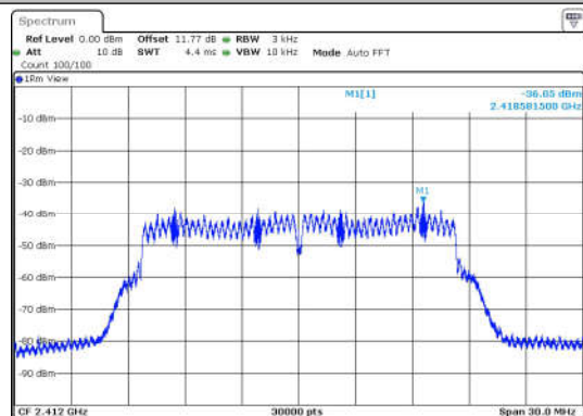
11G-Ant1-2412-PASS
