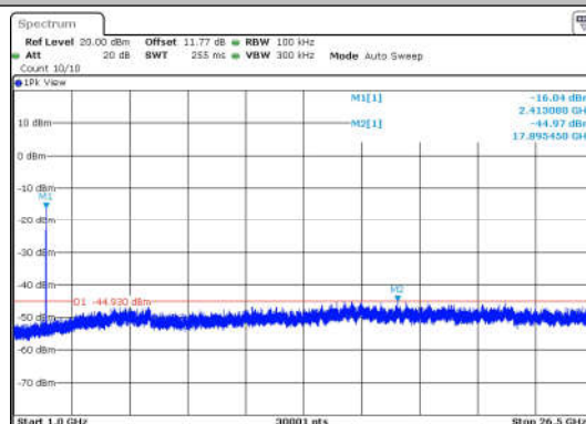
11G-Ant1-2412-1000~26500-PASS
