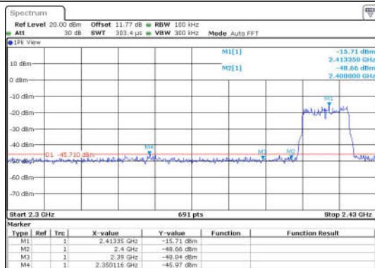
11G-Ant1-2412-PASS
