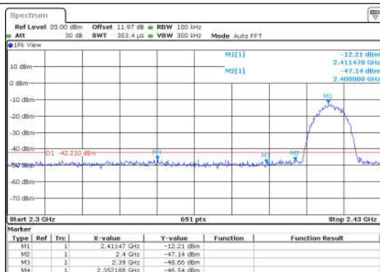
11B-Ant1-2412-PASS
