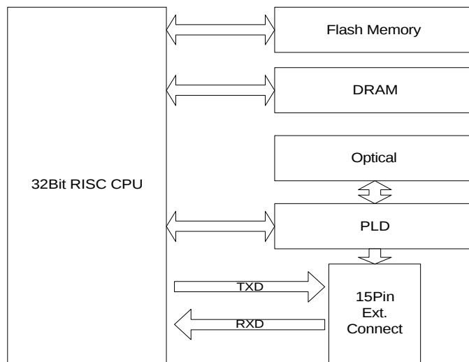
Block Diagram of Finger
