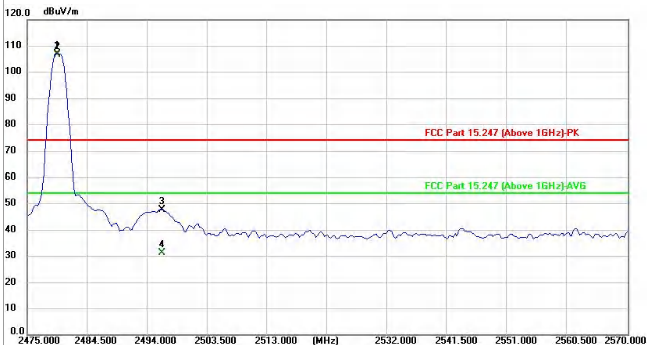
Antennal Polarity&amp; Test Distance: Horizontal at 3 M
