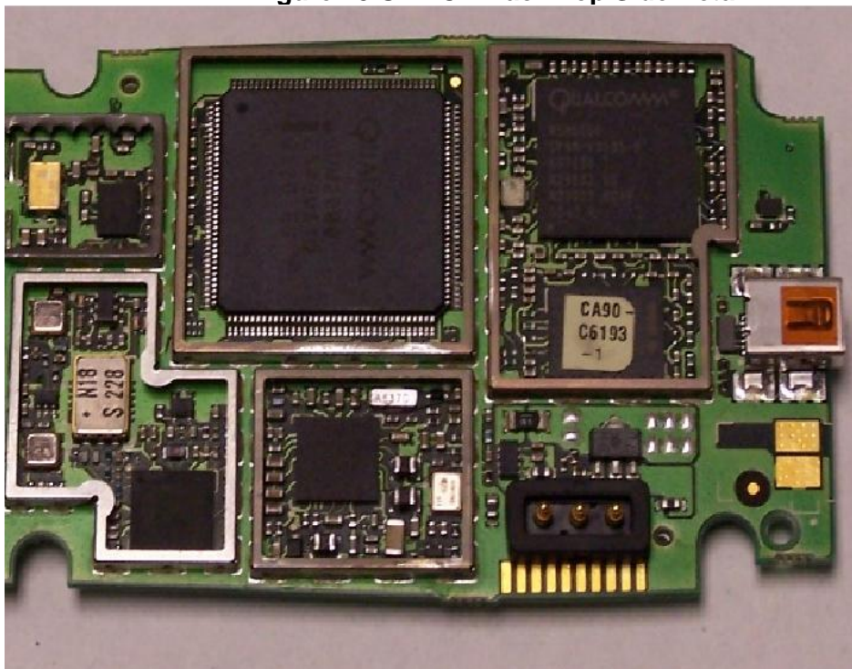
Figure 13 UT PCB Back Top Side Detail
