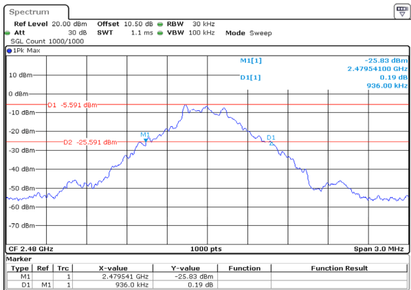
GFSK_High 0.936MHz
