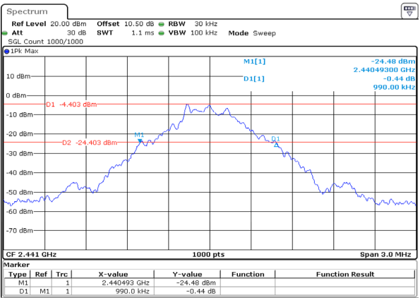
GFSK_Middle 0.990MHz
