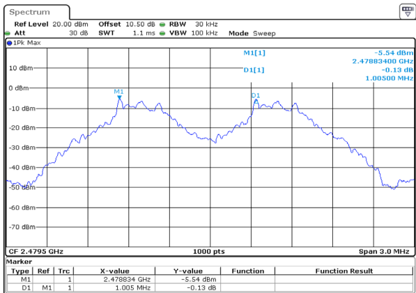
GFSK_High 1.005MHz
