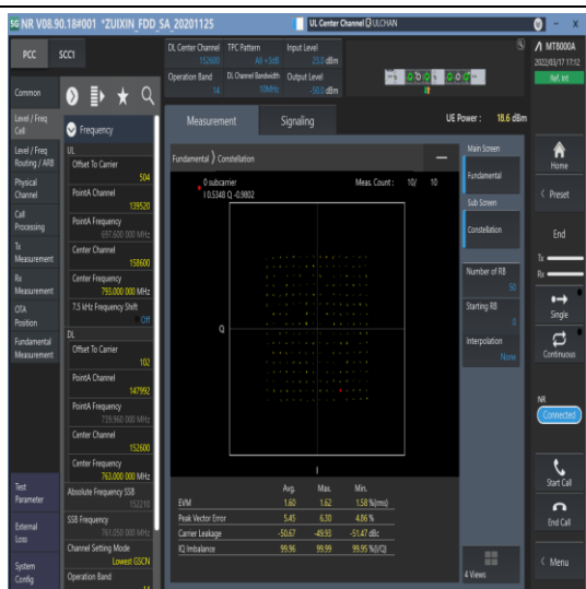
1-N14-15-10-M-5-DFT-256QAM-Outer_Full-50@0-Ant t1-see graph-PASS
