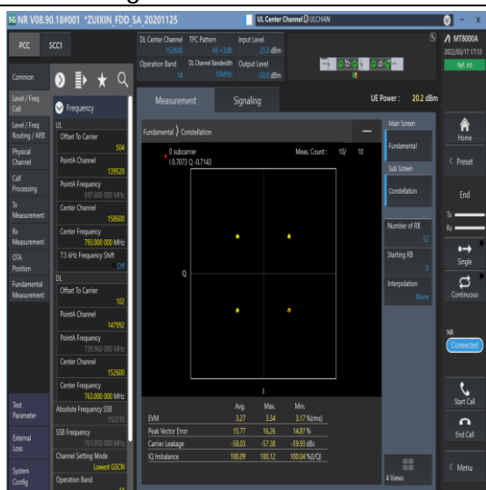
1-N14-15-10-M-6-CP-QPSK-Outer_Full-52@0-Ant1 -see graph-PASS
