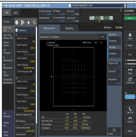
1-N14-15-10-M-8-CP-64QAM-Outer_Full-52@0-Ant 1-see graph-PASS
