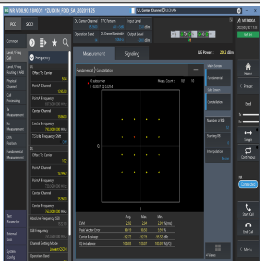
1-N14-15-10-M-7-CP-16QAM-Outer_Full-52@0-Ant1 see graph-PASS
