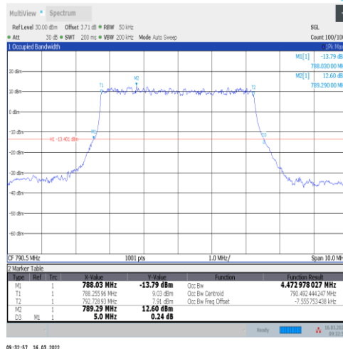
1-N14-15-5-L-2-DFT-PI2BPSK-Outer_Full-25@0-Ant1-4 1-4.473-5.000-≤5-PASS
