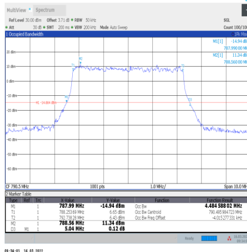
1-N14-15-5-L-4-DFT-64QAM-Outer_Full-25@0-Ant1-4 -4.485-5.040-≤5-PASS
