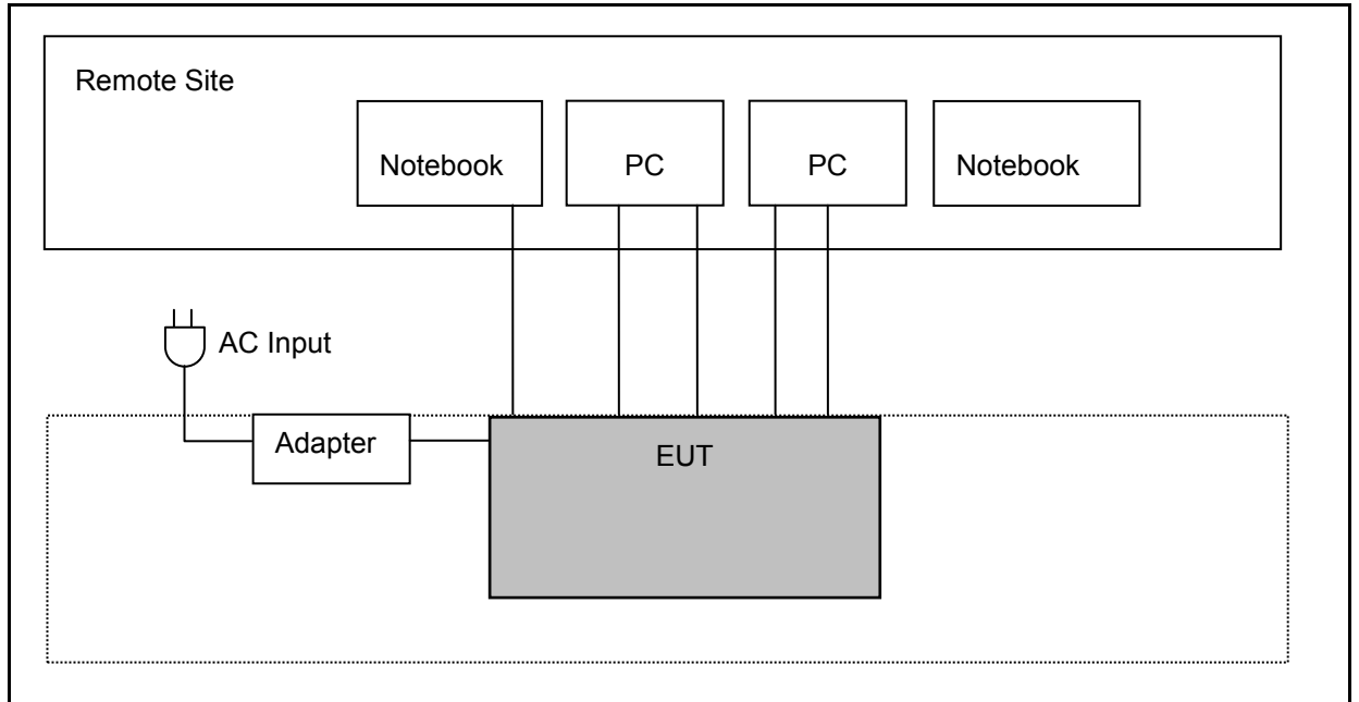
Conducted Emissions
