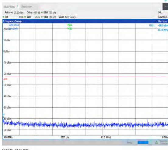
1-N2--15-20-M-1-DFT-PI2BPSK-Inner_1RB_Left-1 @1-30-1000-Ant1--59.85--23-PASS
