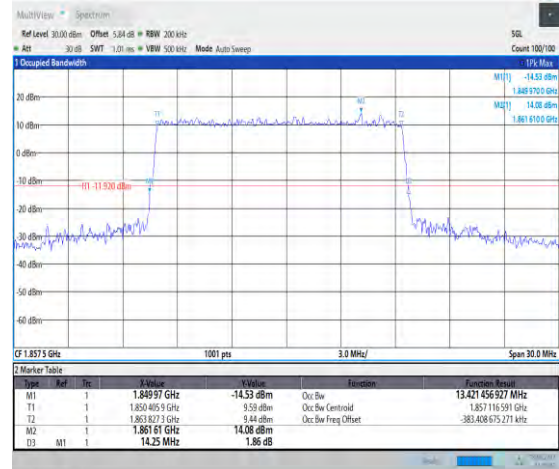
1-N2--15-15-L-4-DFT-64QAM-Outer_Full-75@0-Ant1 -13.421-14.250-≤15-PASS
