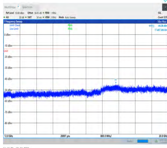
1-N2--15-20-M-1-DFT-PI2BPSK-Inner_1RB_Left-1@ 1-12000-20000-Ant1--44.38--13-PASS
