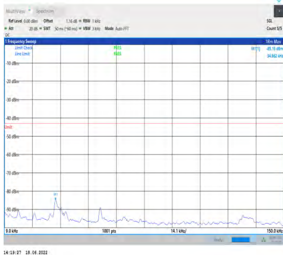
1-N2--15-20-M-1-DFT-PI2BPSK-Inner_1RB_Left-1 @1-0.009-0.15-Ant1--85.16--43-PASS
