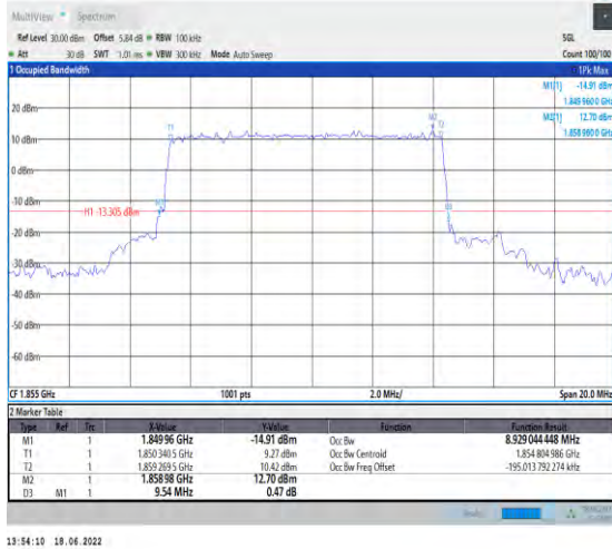
1-N2--15-10-L-2-DFT-PI2BPSK-Outer_Full-50@0-An t1-8.929-9.540≤10-PASS
