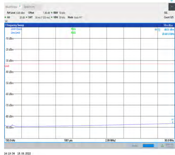
1-N2--15-20-M-1-DFT-PI2BPSK-Inner_1RB_Left-1@ 1-0.15-30-Ant1--86.51--33-PASS
