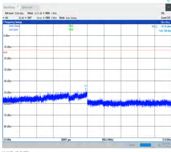
1-N2--15-20-M-1-DFT-PI2BPSK-Inner_1RB_Left-1 @1-3000-12000-Ant1--47.76--13-PASS
