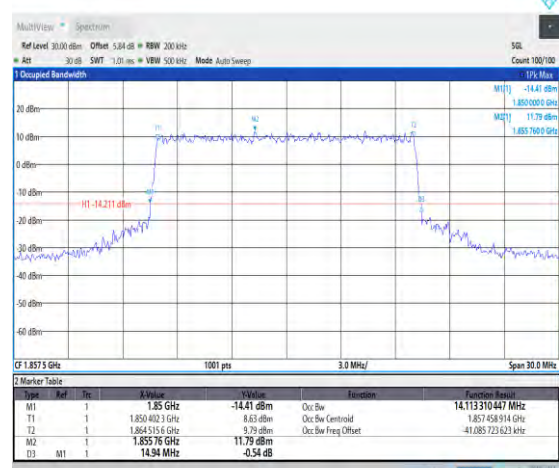
1-N2--15-15-L-6-CP-QPSK-Outer_Full-79@0-Ant1-1 4.113-14.940≤15-PASS
