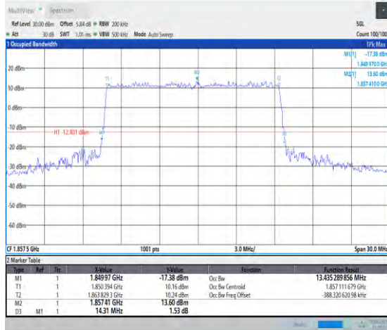
1-N2--15-15-L-3-DFT-16QAM-Outer_Full-75@0-Ant 1-13.435-14.310-≤15-PASS
