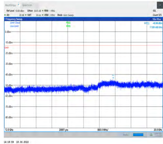
1-N2--15-20-L-1-DFT-PI2BPSK-Inner_1RB_Left-1@ 1-12000-20000-Ant1--43.98--13-PASS
