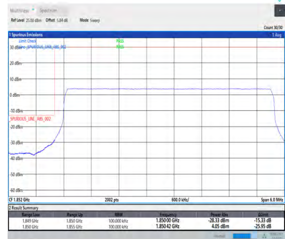
1-N2--15-5-L-6-CP-QPSK-Outer_Full-25@0-Ant1-seegraph-PASS-see graph
