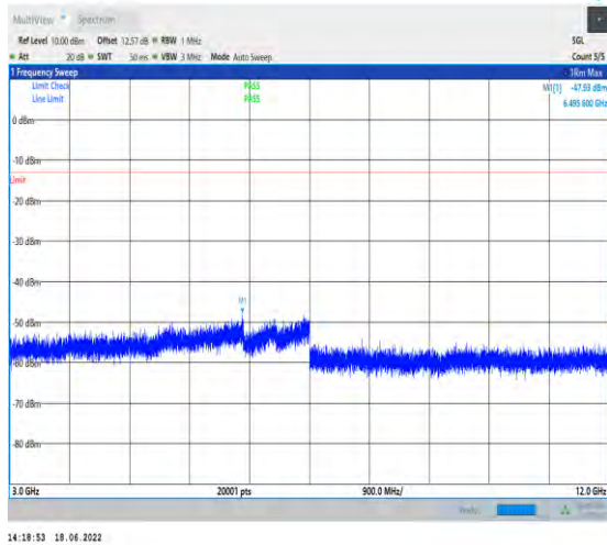
1-N2--15-20-L-1-DFT-PI2BPSK-Inner_1RB_Left-1@ 1-3000-12000-Ant1--47.93--13-PASS
