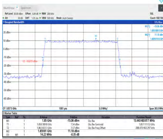
1-N2--15-15-L-5-DFT-256QAM-Outer_Full-75@0-An t1-13.443-14.220-≤15-PASS
