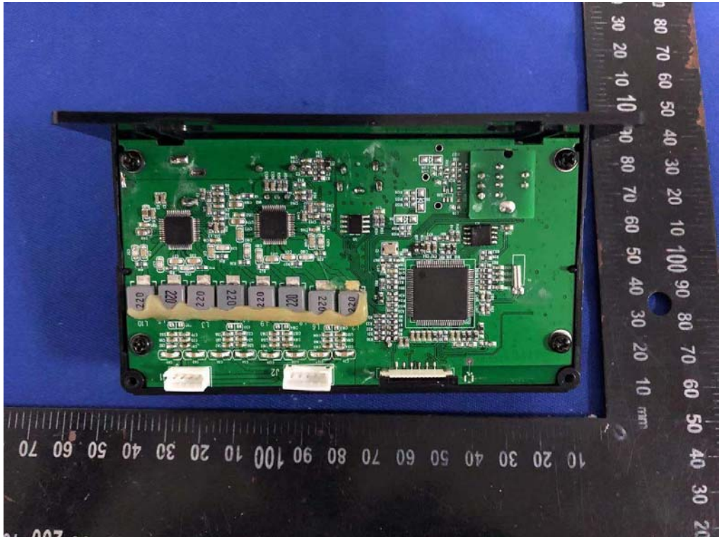
Internal Photos M/N: R-4B II NA Soundbar
