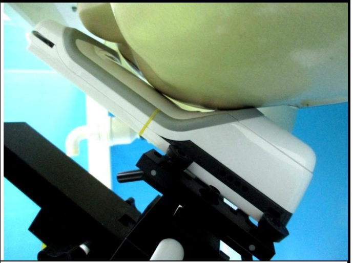
Body - Left Face of EUT with 0 cm Gap
