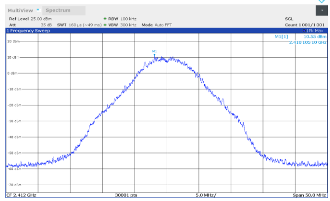
Figure 8.4-24: TSM-Bandwidth 10MHz conducted spurious emission reference level, 2412 MHz
