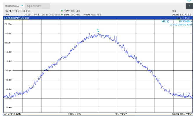
Figure 8.4-26: TSM-Bandwidth 10MHz conducted spurious emission reference level, 2442 MHz
