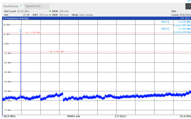
Figure 8.4-23: TSM-Bandwidth 10MHz conducted spurious emission, 2412 MHz
