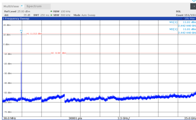
Figure 8.4-25: TSM-Bandwidth 10MHz conducted spurious emission, 2442 MHz
