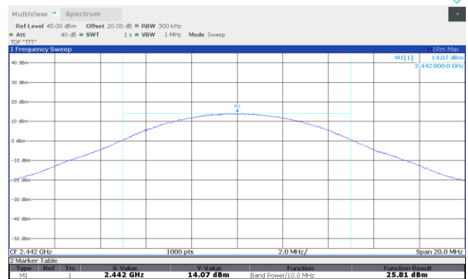
Figure 8.3-8: TSM-Bandwidth 10MHz Conducted output power, 2442 MHz
