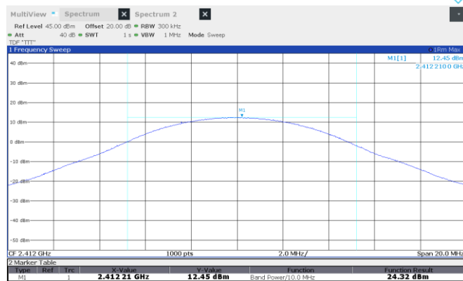
Figure 8.3-7: TSM-Bandwidth 10MHz Conducted output power, 2412 MHz
