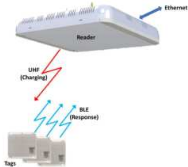
Figure 2 - Reader's functionality
