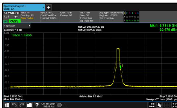
Figure 316 - B (Core 1) 802.11a SP 6695 MHz (CH149)
