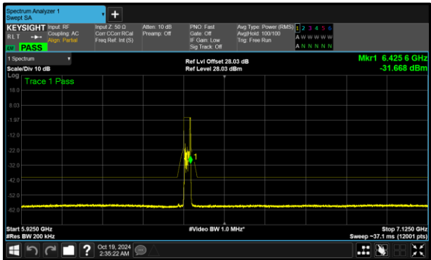
Figure 343 - B (Core 1) 802.11ax HE20 RU26 SP 6415 MHz (CH93)
