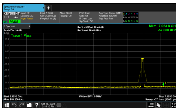
Figure 308 - B (Core 1) 802.11a LPI 6875 MHz (CH185)
