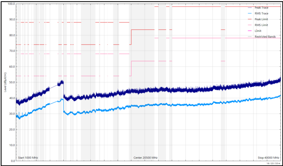
Figure 295 - 6695 MHz (CH149), HE20, SU, CDD, Core 0 + Core 1, 1 GHz to 40 GHz, Horizontal
