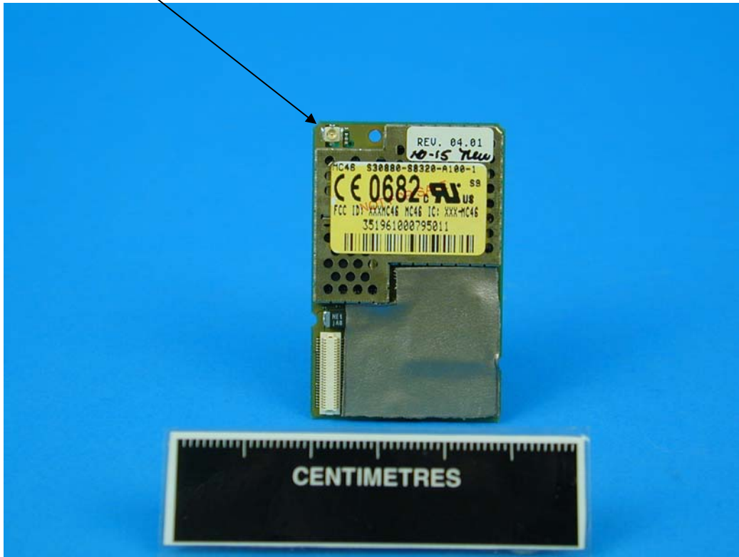
700C – internal Antenna connector
