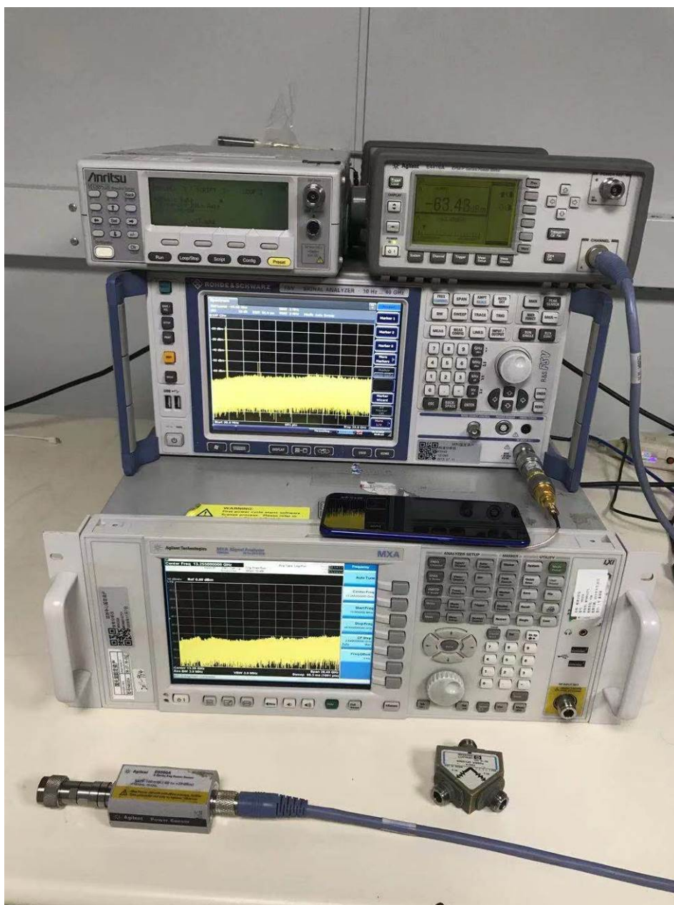
RF Conducted Test setup (BT/WIFI)
