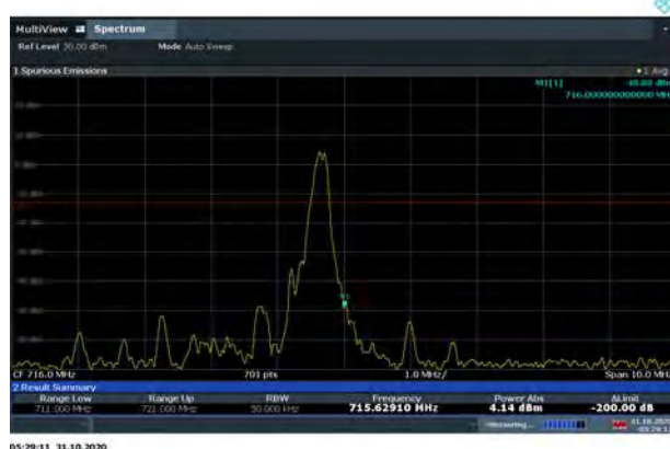
LTE Band 85 16QAM 5MHz CH-High, 1 RB
