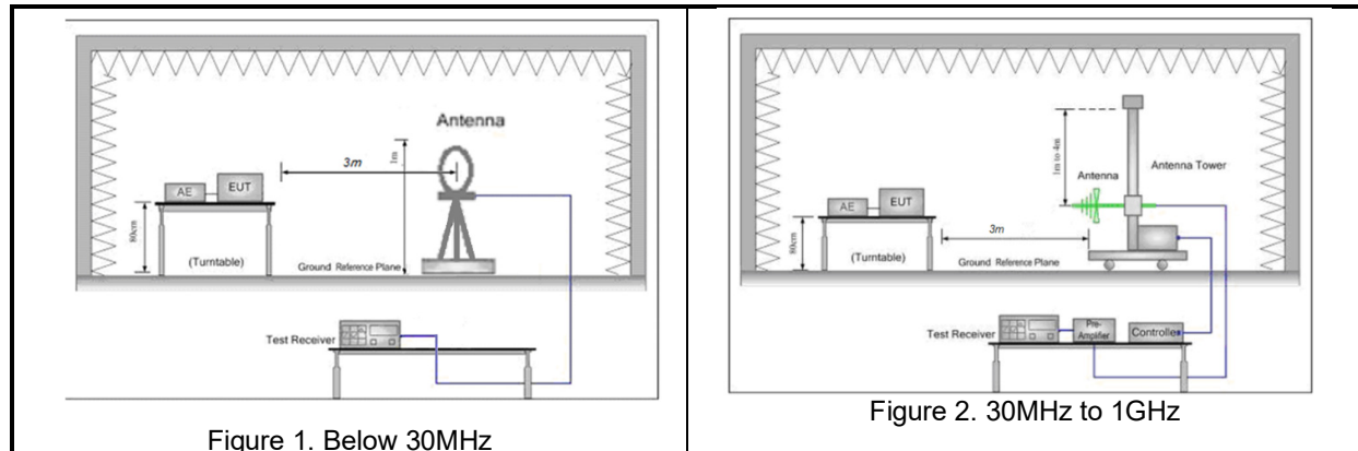
Figure 1. Below 30MHz
