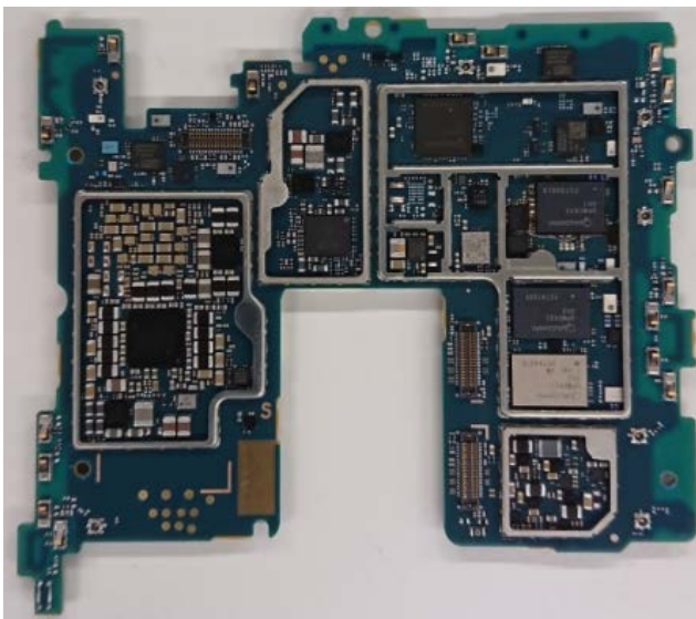
Internal PWB without Shield cases (Rear-side)
