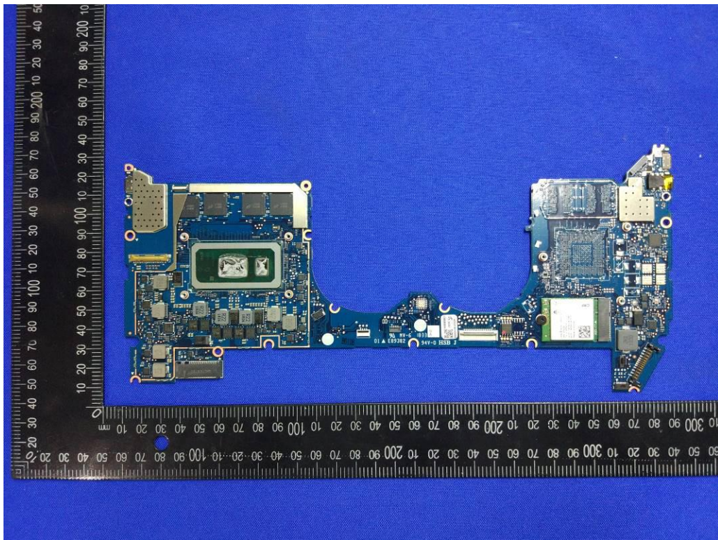
WRT-W19, WRT-W29(without GPU) MAIN BOARD TOP VIEW
