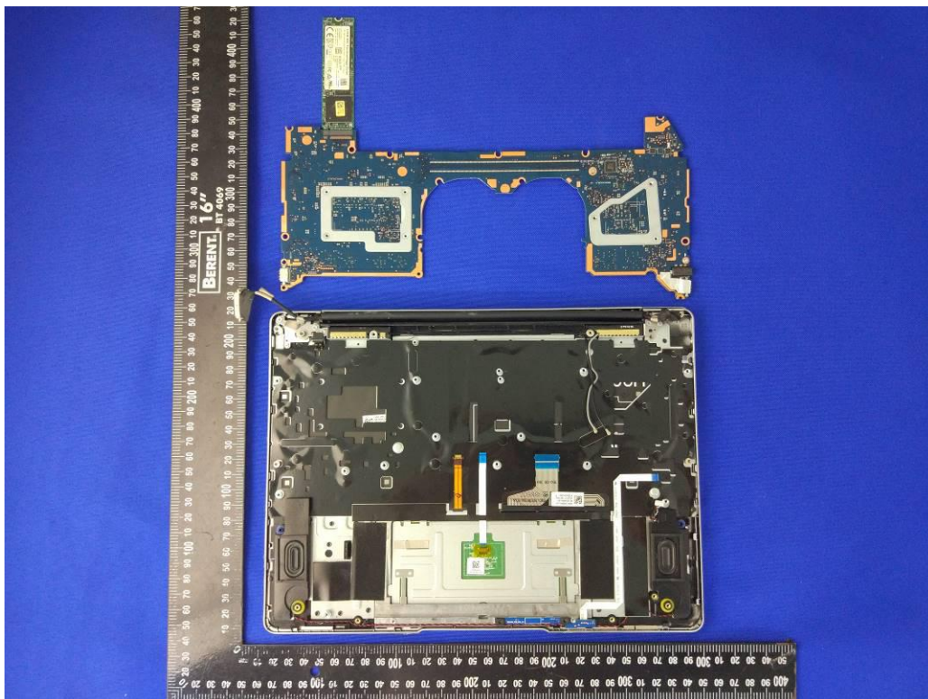
WRT-W19, WRT-W29 UNCOVER VIEW
