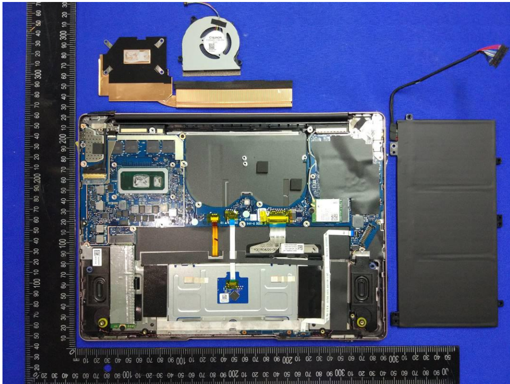
WRT-W19, WRT-W29(without GPU) UNCOVER VIEW
