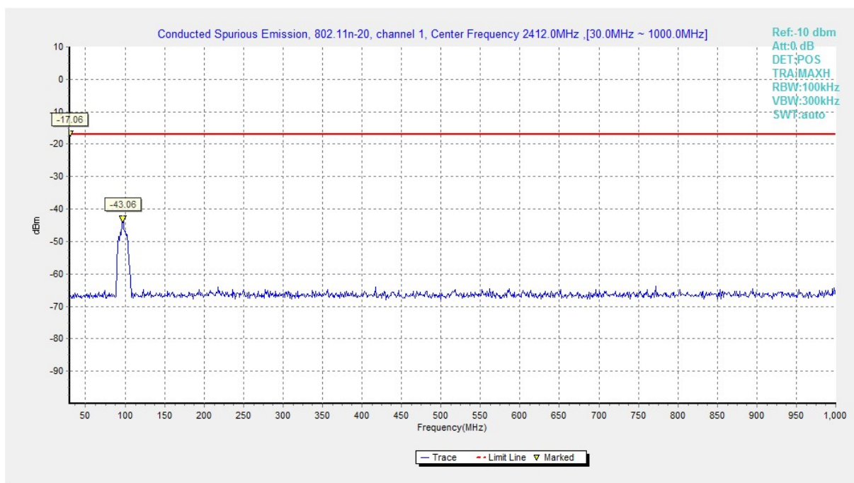
Fig.A.6.1.50 Conducted Spurious Emission (802.11n-HT20, Ch1, 30 MHz-1 GHz)
