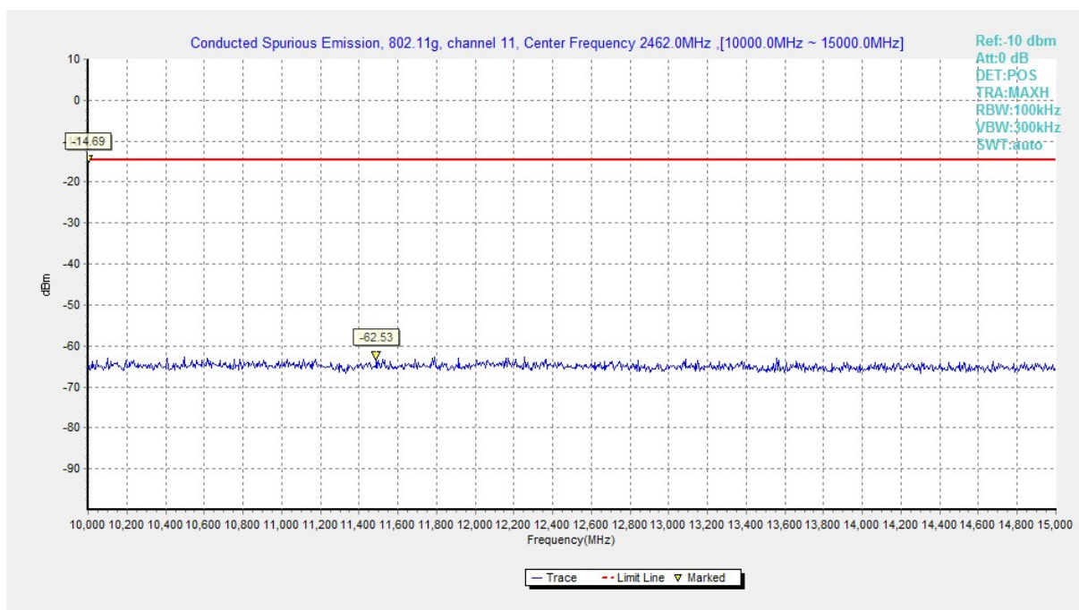
Fig.A.6.1.46 Conducted Spurious Emission (802.11g, Ch11, 10 GHz-15 GHz)
