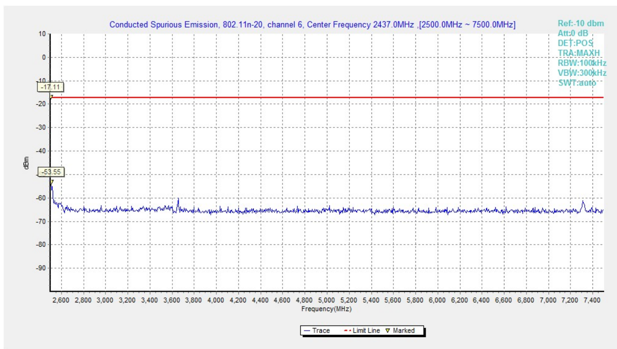
Fig.A.6.1.60 Conducted Spurious Emission (802.11n-HT20, Ch6, 2.5 GHz-7.5 GHz)
