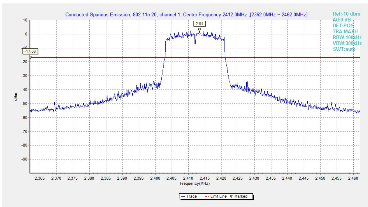
Fig.A.6.1.49 Conducted Spurious Emission (802.11n-HT20, Ch1, Center Frequency)
