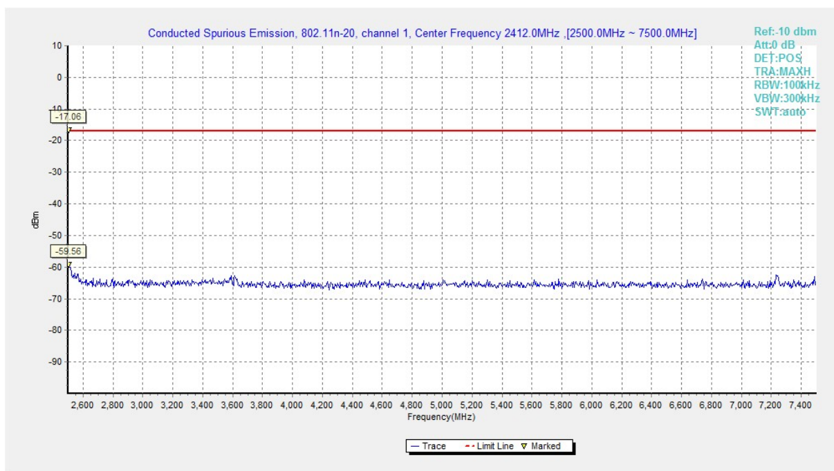
Fig.A.6.1.52 Conducted Spurious Emission (802.11n-HT20, Ch1, 2.5 GHz-7.5 GHz)
