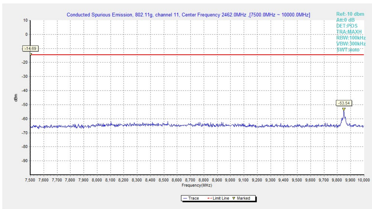
Fig.A.6.1.45 Conducted Spurious Emission (802.11g, Ch11, 7.5 GHz-10 GHz)
