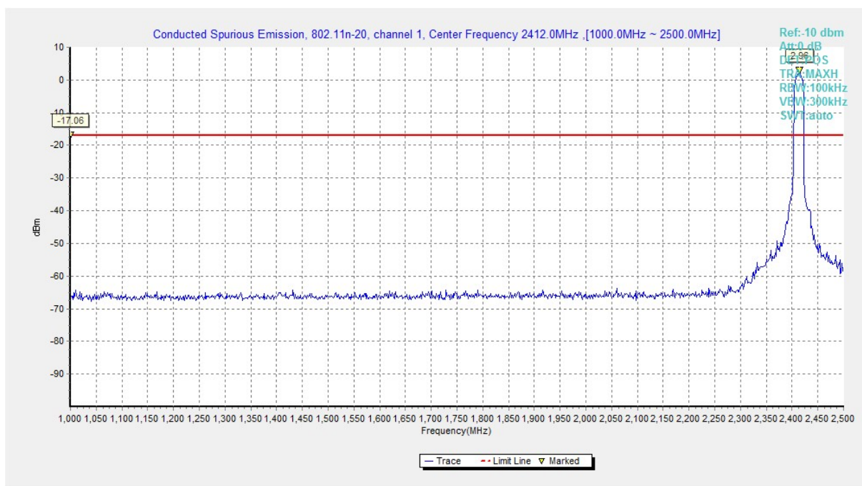
Fig.A.6.1.51 Conducted Spurious Emission (802.11n-HT20, Ch1, 1 GHz-2.5 GHz)
