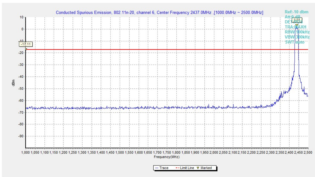
Fig.A.6.1.59 Conducted Spurious Emission (802.11n-HT20, Ch6, 1 GHz-2.5 GHz)
