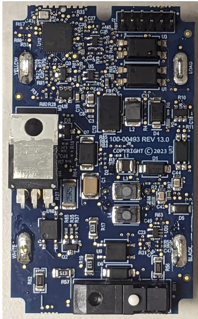
Photograph 4 – Top View of the Load PCB
