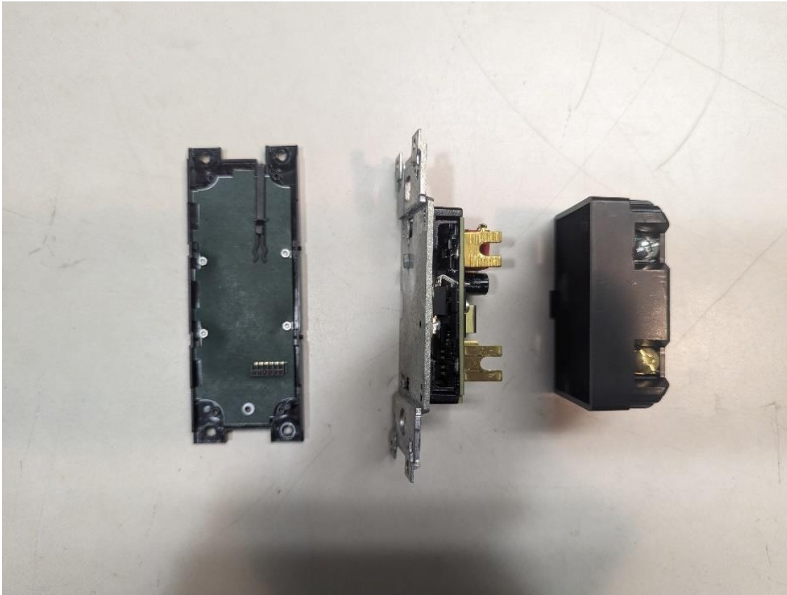
Photograph 6 – Radio PCB, Load PCB, and Enclosure Housing
