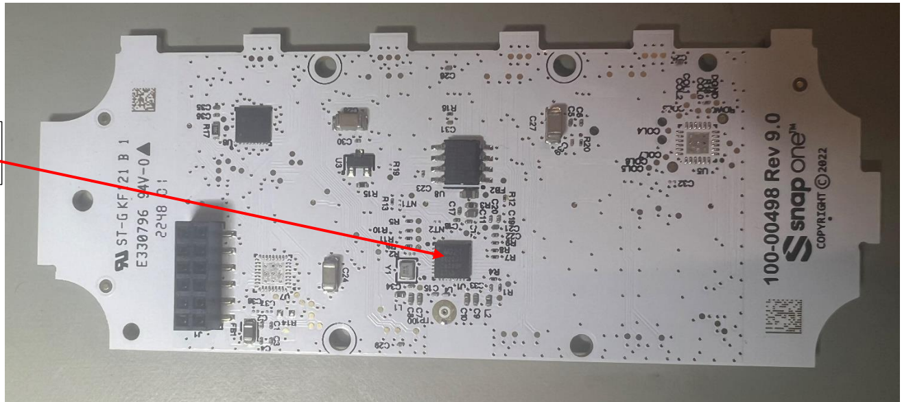
Photograph 2 – Top view of Radio PCB
