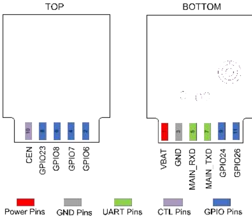
Figure 2: Pin Assignment
