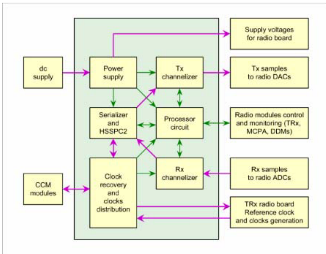
Functional block diagram of the TRM
