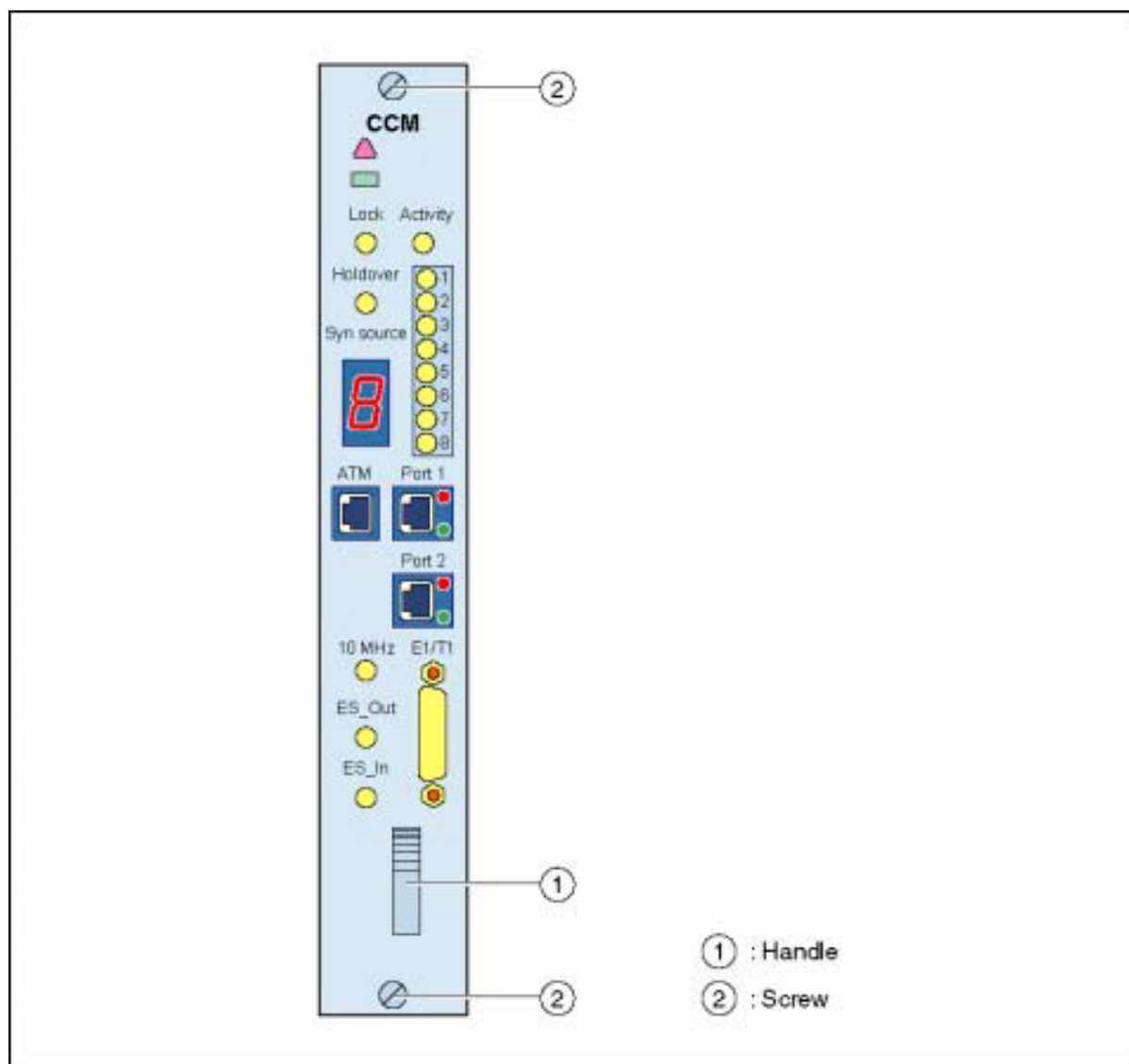
Front view of the CCM
