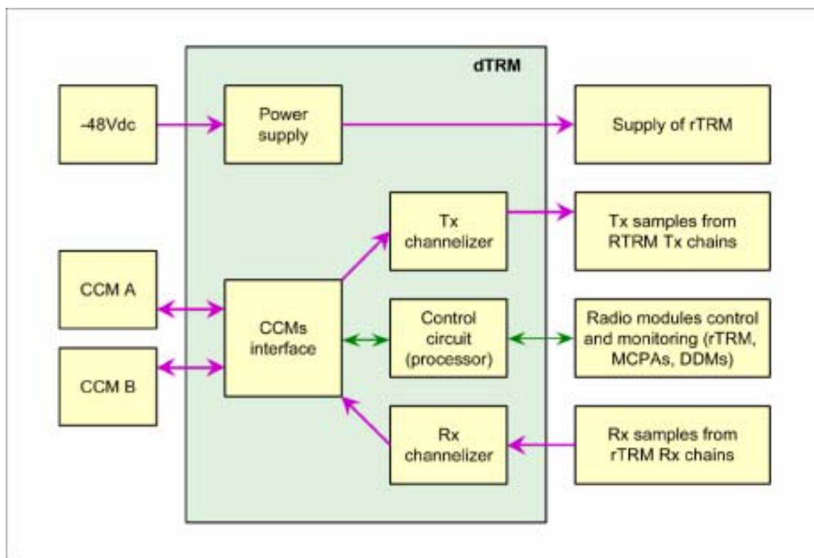
Block diagram of the dTRM board
