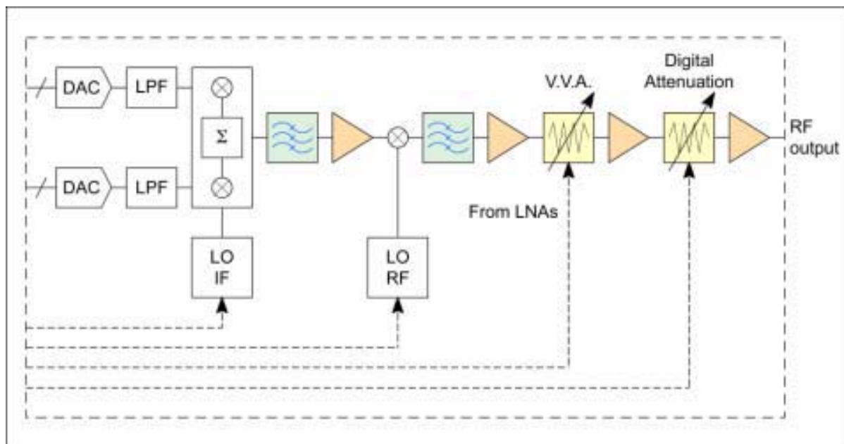
Block diagram of the rTRM transmit part
