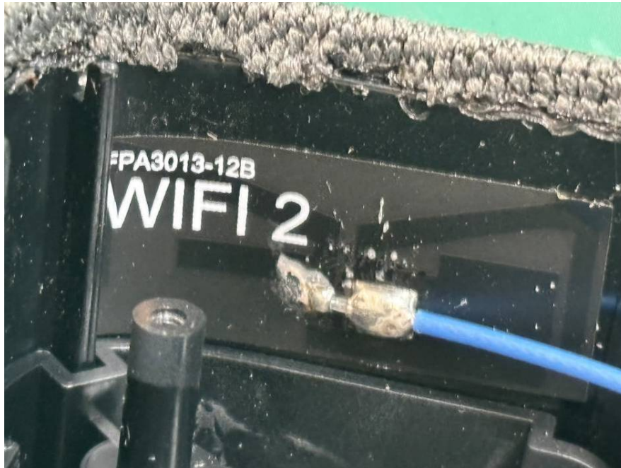
Wi-Fi ANT2
