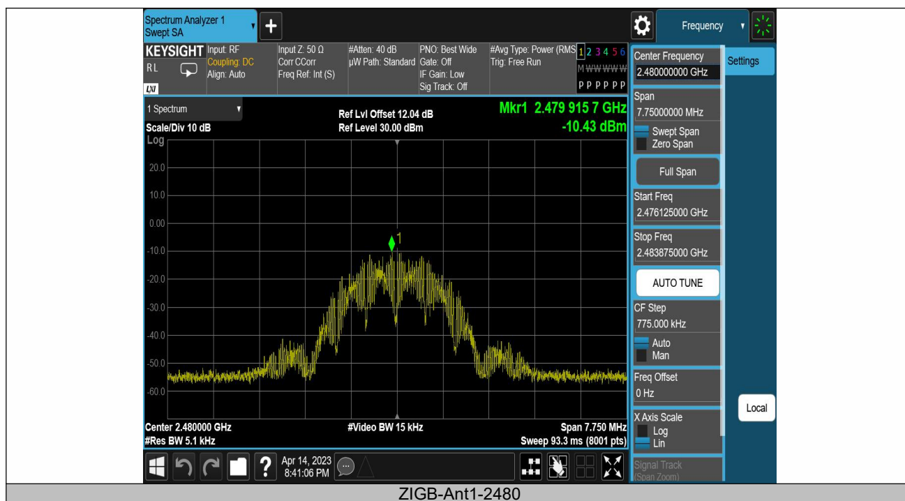
ZIGB-Ant1-2480
