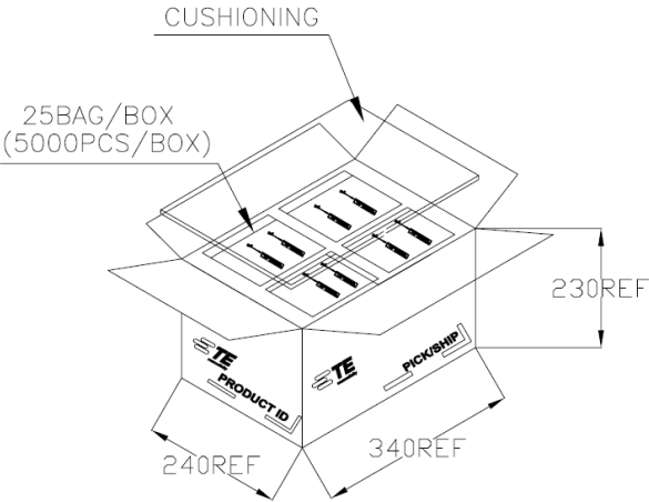
200PCS/BAG DESICCANT:1PCS/BAG
