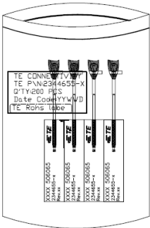
200PCS/BAG DESICCANT:1PCS/BAG
