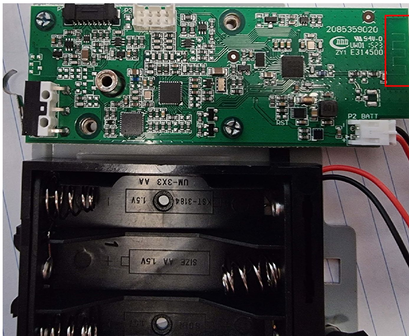
Cartridge Mortise Bluetooth Antenna Location (Red)
