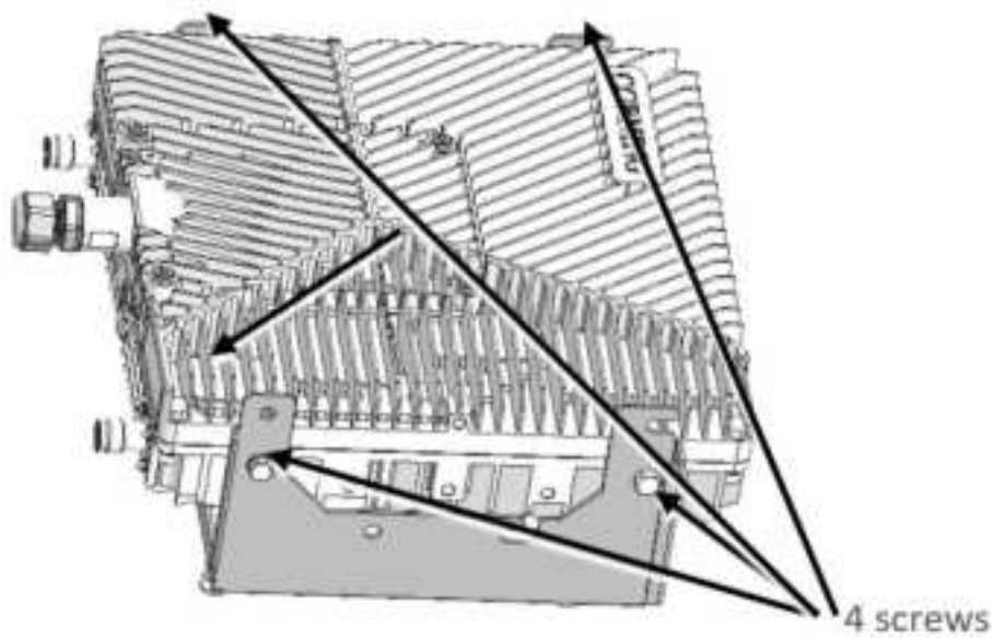
Figure 37-4 screws
