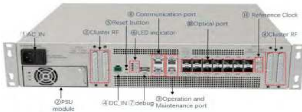
Figure 12. DCU Interface (front view)
