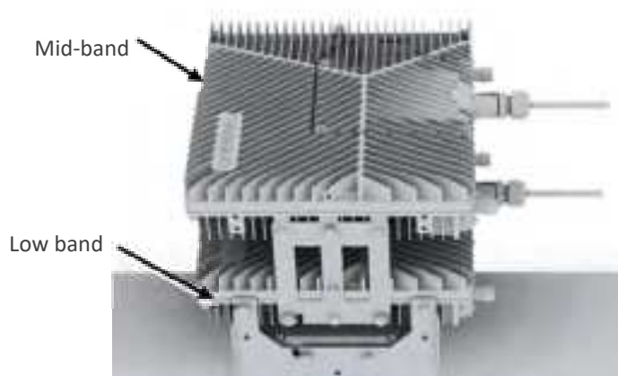
Figure 39 Combiner in the bracket
