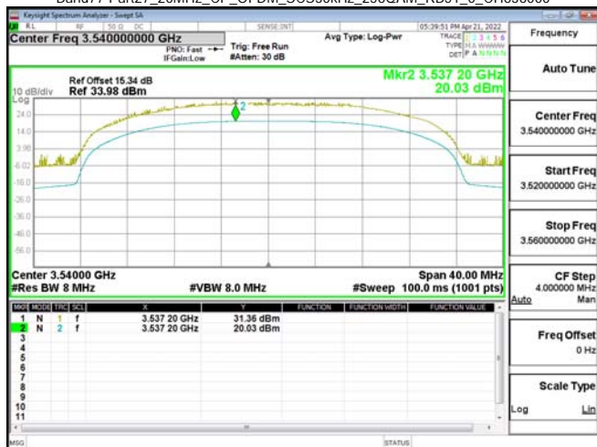
Band77-Part27_20MHz_CP_OFDM_SCS30kHz_256QAM_RB51_0_CH636000
