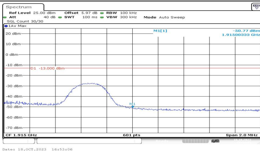
Band25-5MHz-QPSK-26665-1RB#0-PASS
