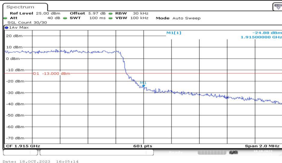
Band25-1.4MHz-16QAM-26683-6RB#0-PASS
