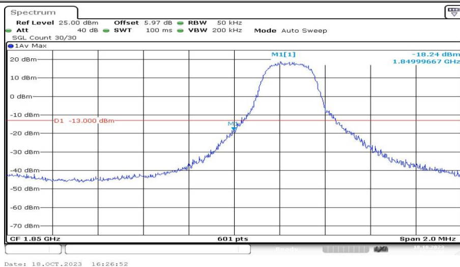
Band25-3MHz-QPSK-26055-1RB#0-PASS
