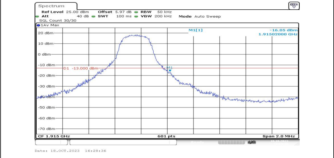
Band25-3MHz-QPSK-26675-1RB#14-PASS
