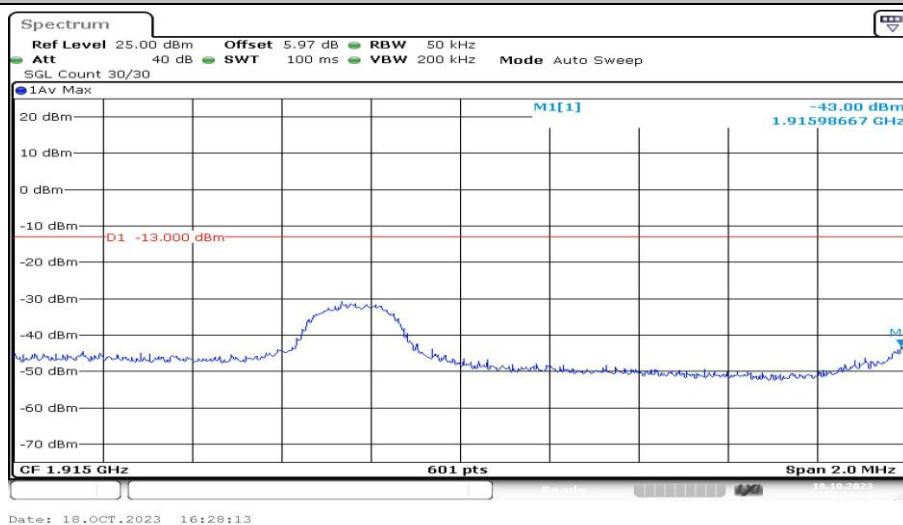
Band25-3MHz-QPSK-26675-1RB#0-PASS
