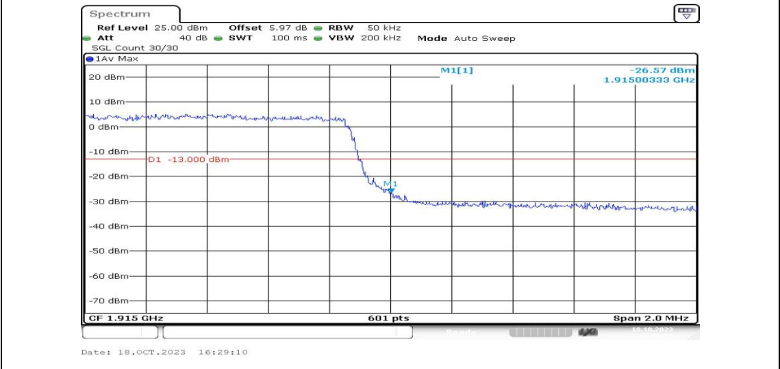
Band25-3MHz-16QAM-26675-15RB#0-PASS
