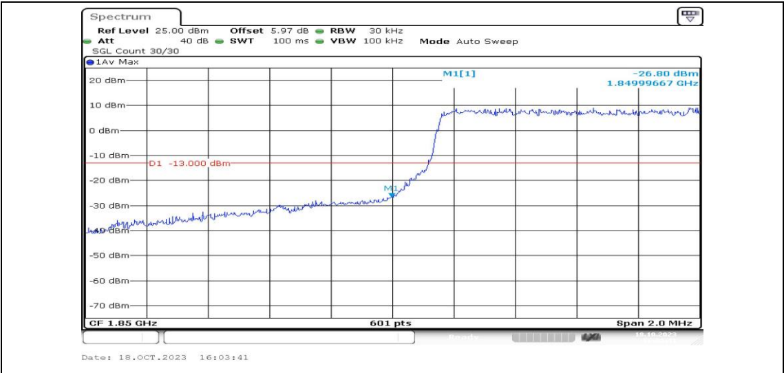
Band25-1.4MHz-QPSK-26047-6RB#0-PASS
