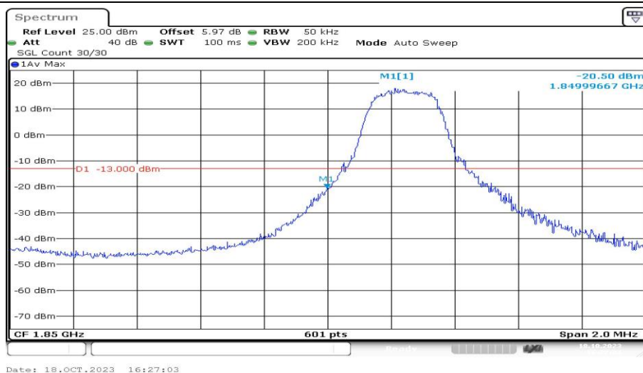
Band25-3MHz-16QAM-26055-1RB#0-PASS
