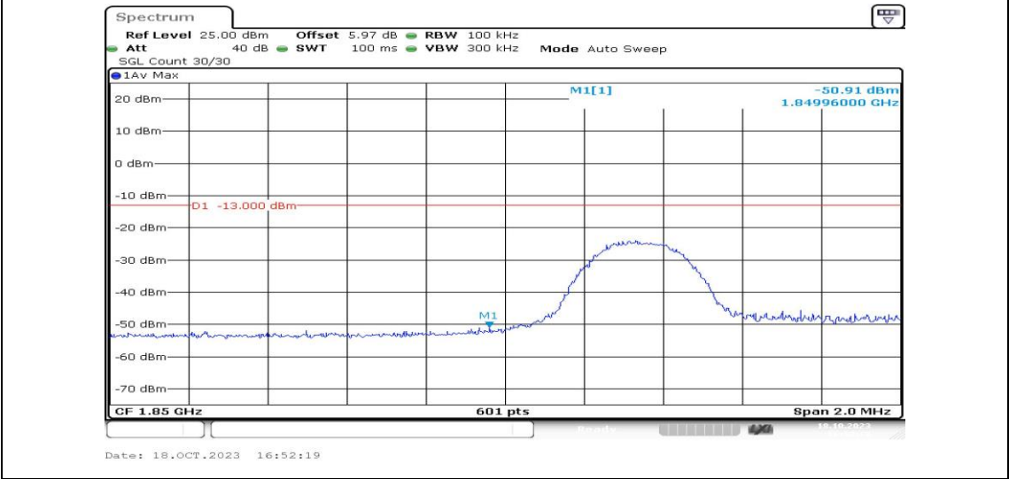
Band25-5MHz-16QAM-26065-1RB#24-PASS
