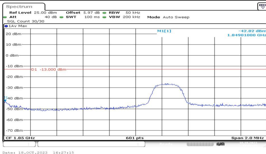
Band25-3MHz-QPSK-26055-1RB#14-PASS
