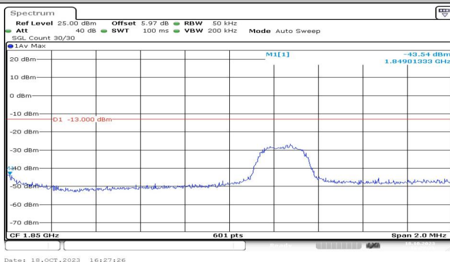
Band25-3MHz-16QAM-26055-1RB#14-PASS
