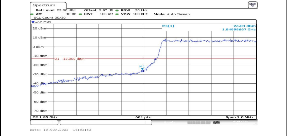
Band25-1.4MHz-16QAM-26047-6RB#0-PASS
