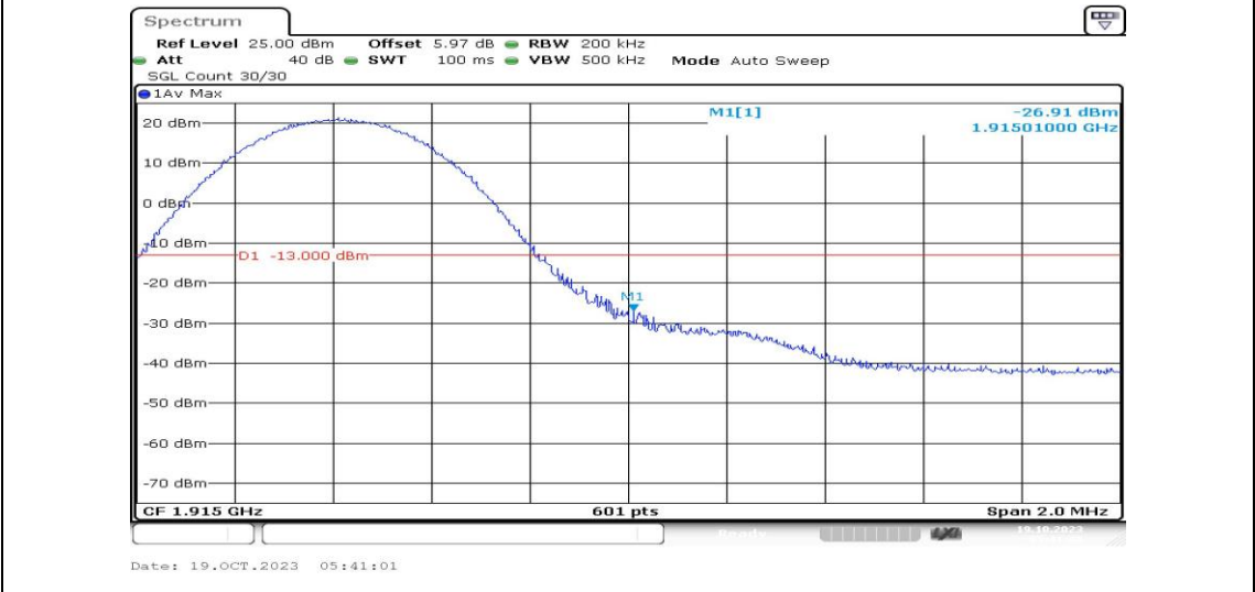
Band25-10MHz-16QAM-26640-1RB#49-PASS
