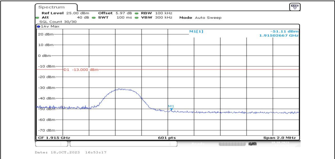
Band25-5MHz-16QAM-26665-1RB#0-PASS
