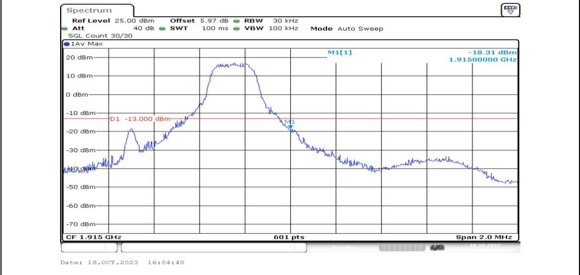
Band25-1.4MHz-QPSK-26683-1RB#5-PASS
