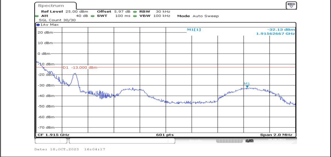
Band25-1.4MHz-QPSK-26683-1RB#0-PASS
