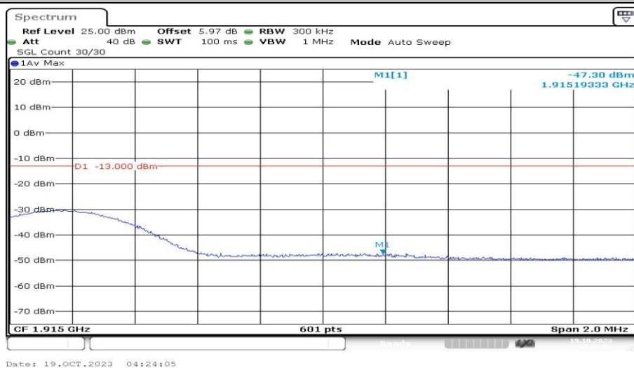
Band25-15MHz-QPSK-26615-1RB#0-PASS
