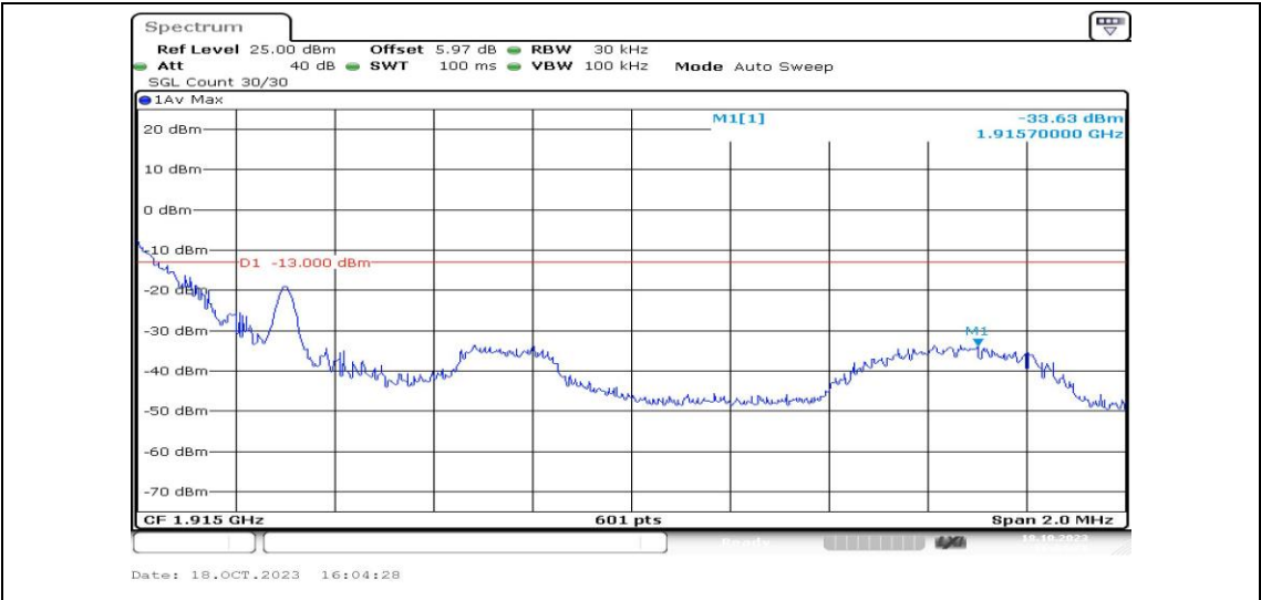
Band25-1.4MHz-16QAM-26683-1RB#0-PASS
