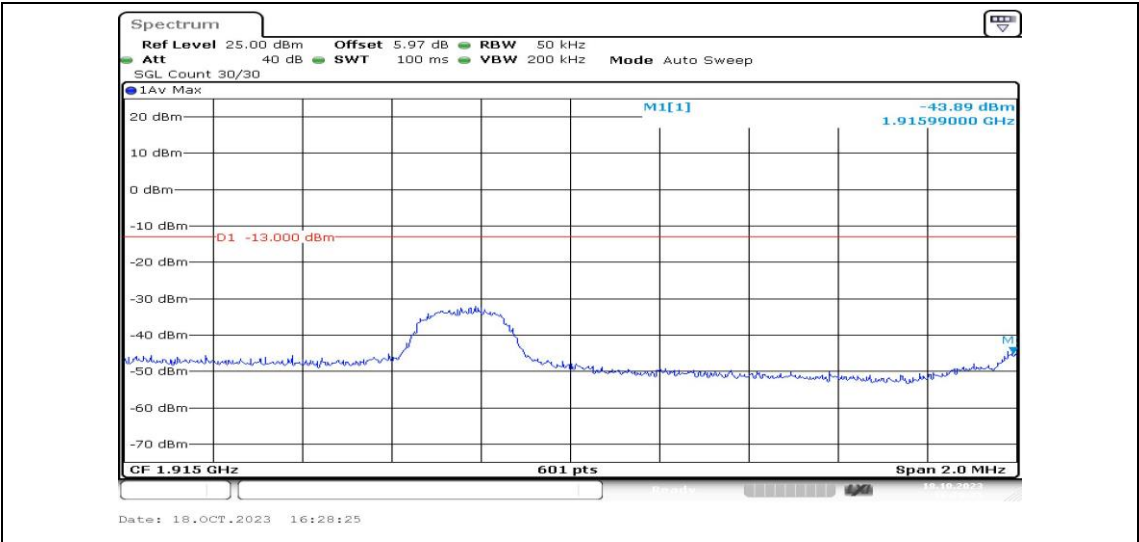
Band25-3MHz-16QAM-26675-1RB#0-PASS
