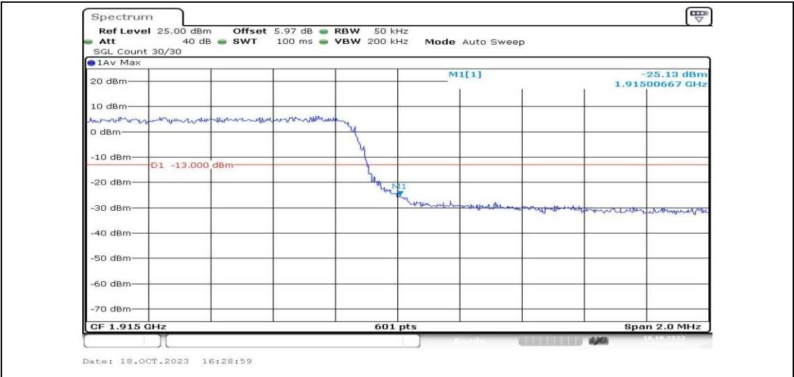
Band25-3MHz-QPSK-26675-15RB#0-PASS
