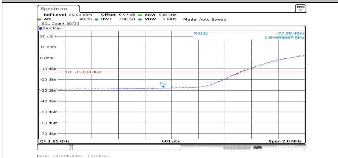
Band25-20MHz-QPSK-26140-100RB#0-PASS
