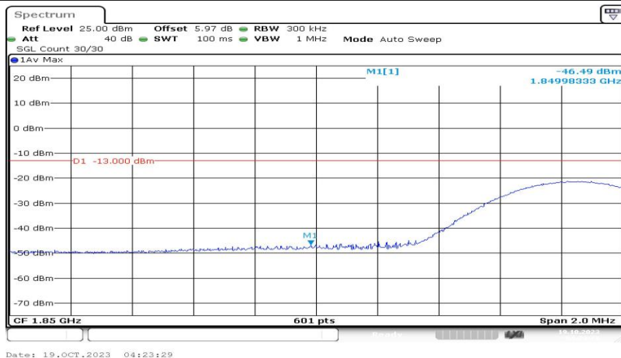
Band25-15MHz-QPSK-26115-1RB#74-PASS
