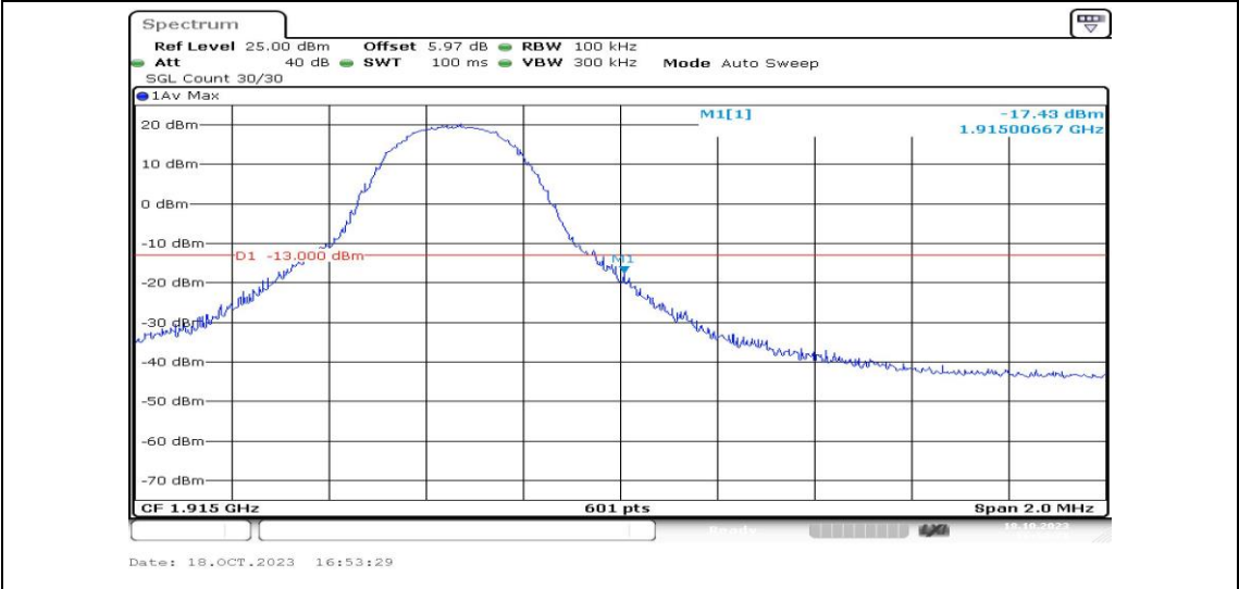
Band25-5MHz-QPSK-26665-1RB#24-PASS
