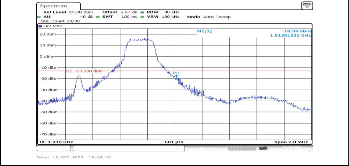
Band25-1.4MHz-16QAM-26683-1RB#5-PASS
