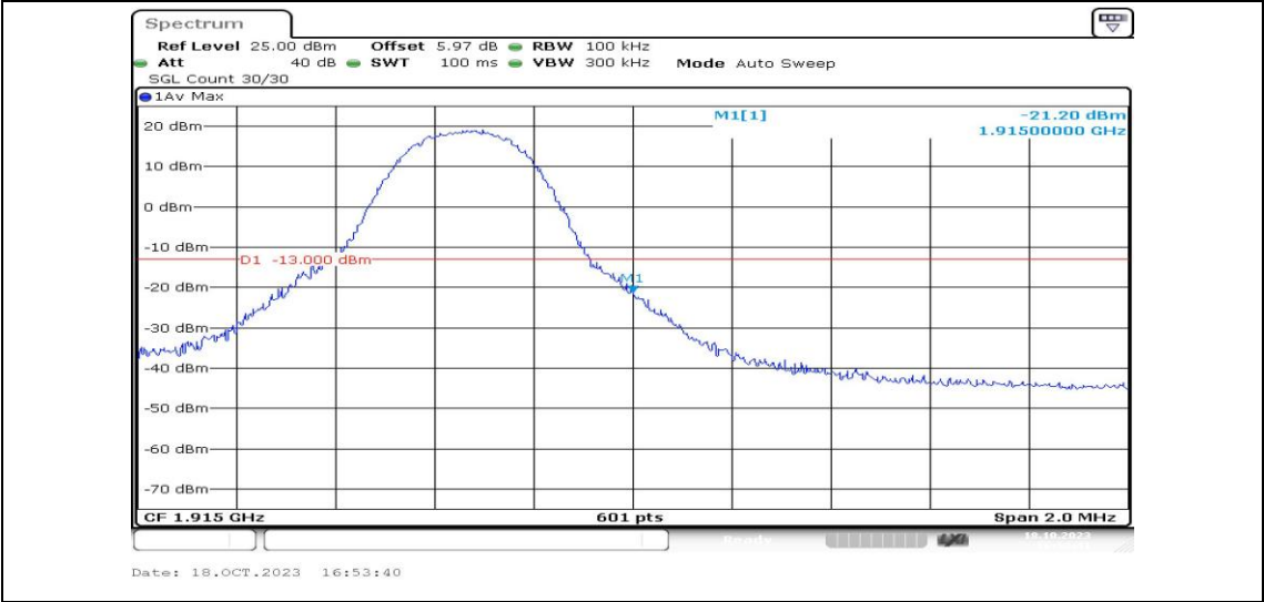
Band25-5MHz-16QAM-26665-1RB#24-PASS
