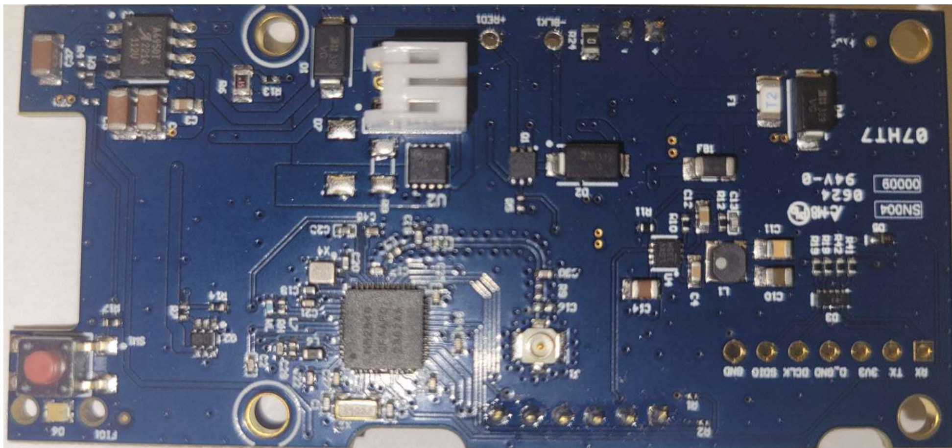
Figure 1: PCBA Front
