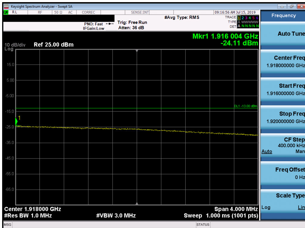
Plot 7-263. Upper Extended Band Edge Plot (Band 25 - 15.0MHz QPSK - Full RB Configuration)
