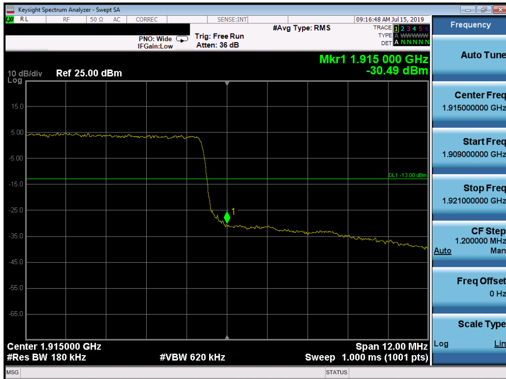
Plot 7-262. Upper Band Edge Plot (Band 25 - 15.0MHz QPSK - Full RB Configuration)
