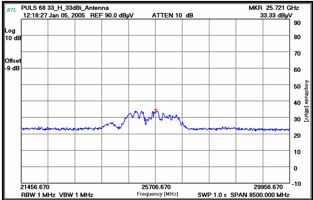
PLOT 7-2 EUT HORN 33DBI ANTENNA 100% DUTY CYCLE PEAK MODE H POL
