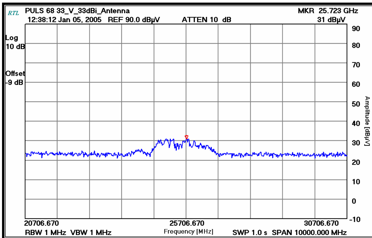
PLOT 7-3 EUT HORN 33DBI ANTENNA 100% DUTY CYCLE PEAK MODE V POL
