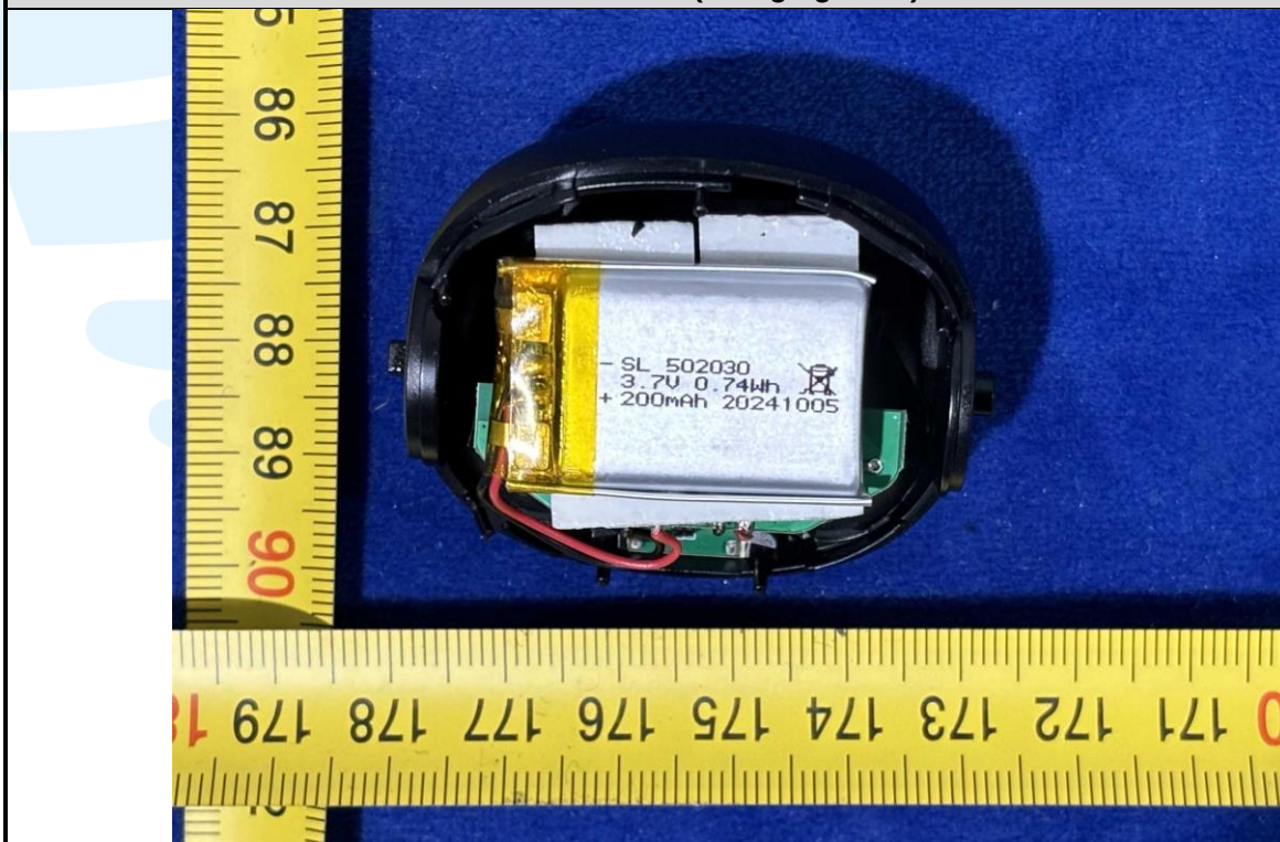
EUT Photo(Charging Case)
