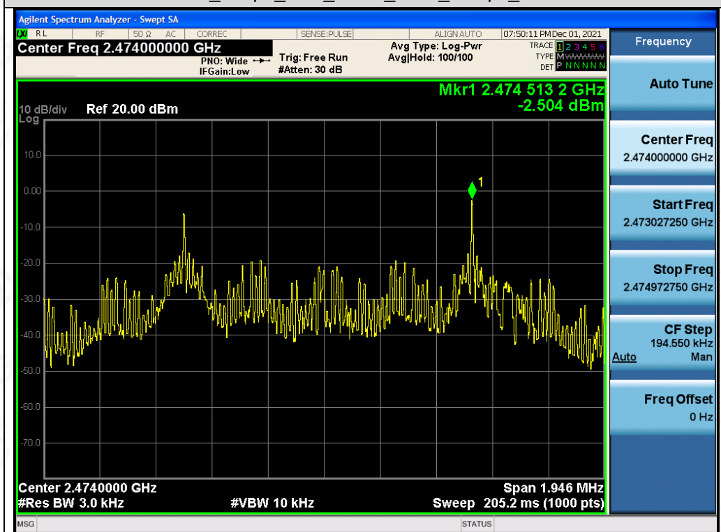
Test_Graph_FSK_ANT1_2474_2Mbps_PSD
