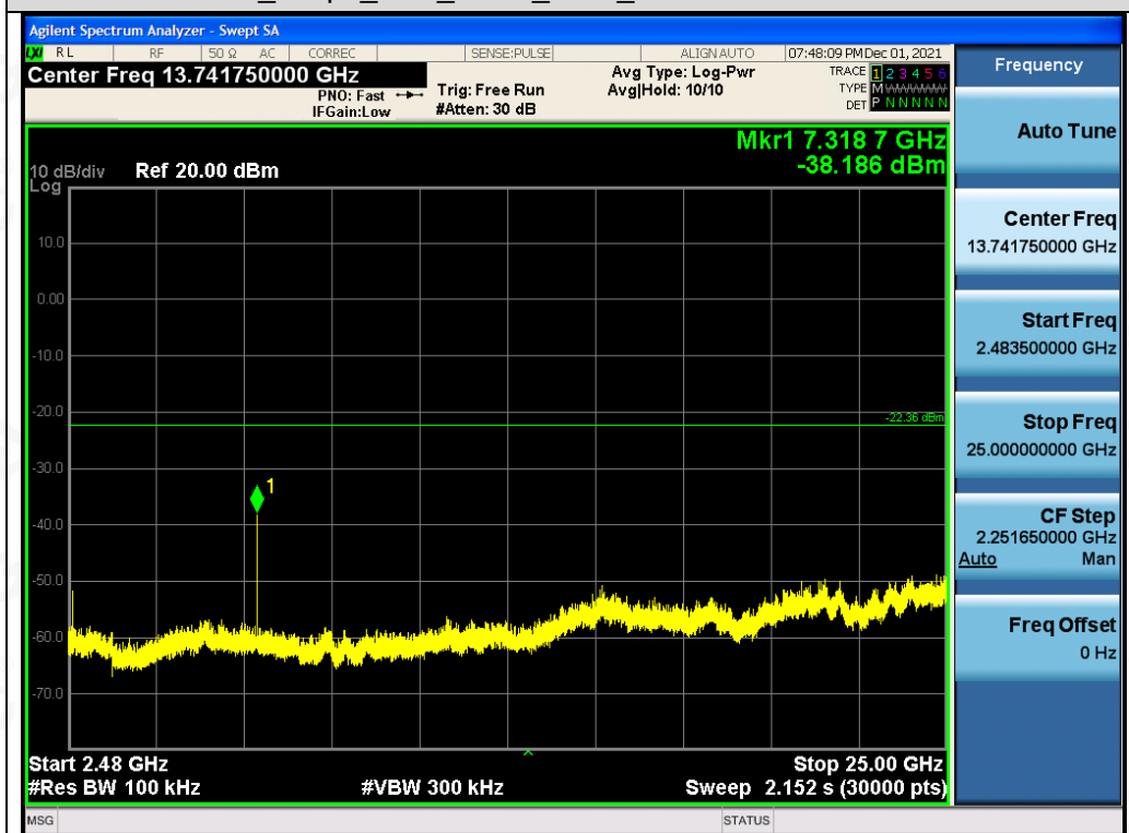
Test_Graph_FSK_ANT1_2440_Higher Band Emissions
