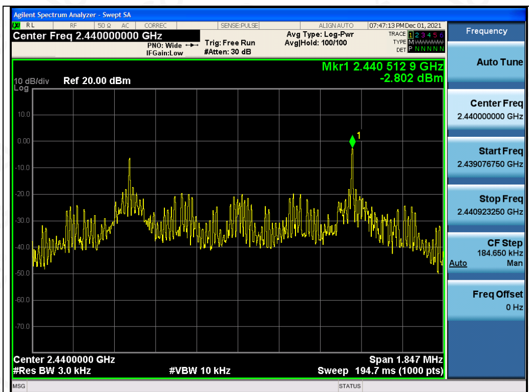
Test_Graph_FSK_ANT1_2440_2Mbps_PSD
