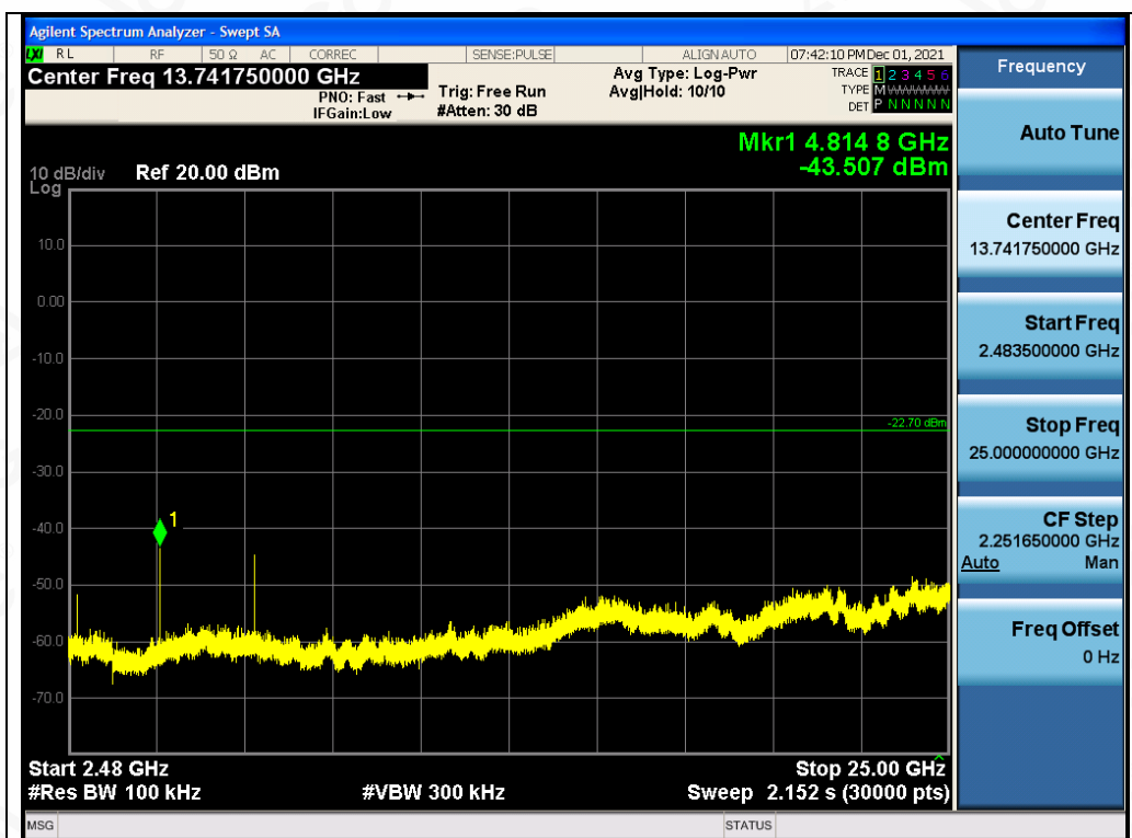
Test_Graph_FSK_ANT1_2408_Higher Band Emissions
