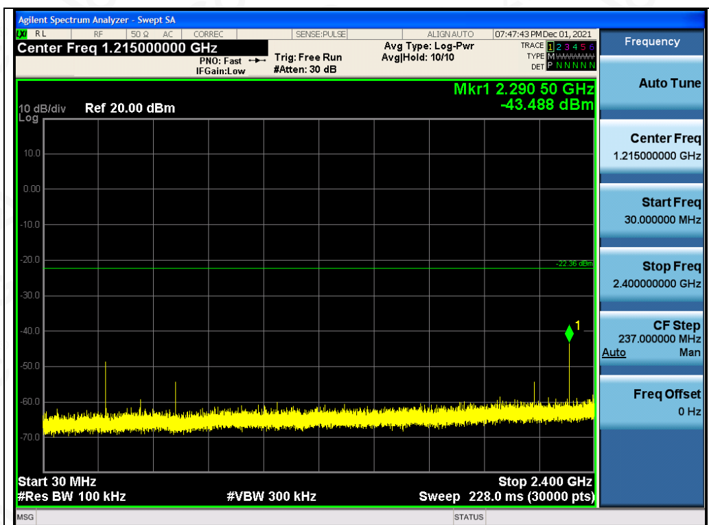
Test_Graph_FSK_ANT1_2440_Lower Band Emissions
