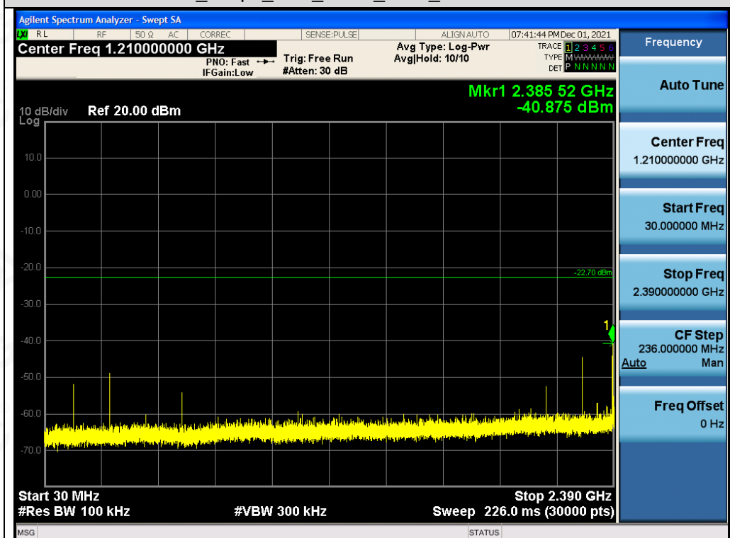
Test Graph FSK ANT1 2408 Lower Band Emissions
