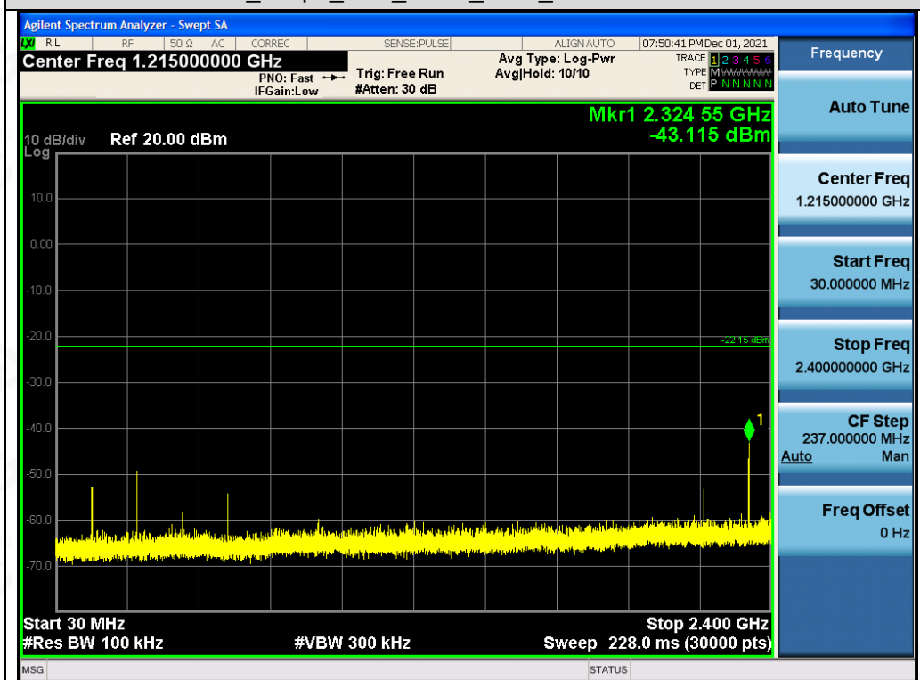
Test_Graph_FSK_ANT1_2474_Lower Band Emissions
